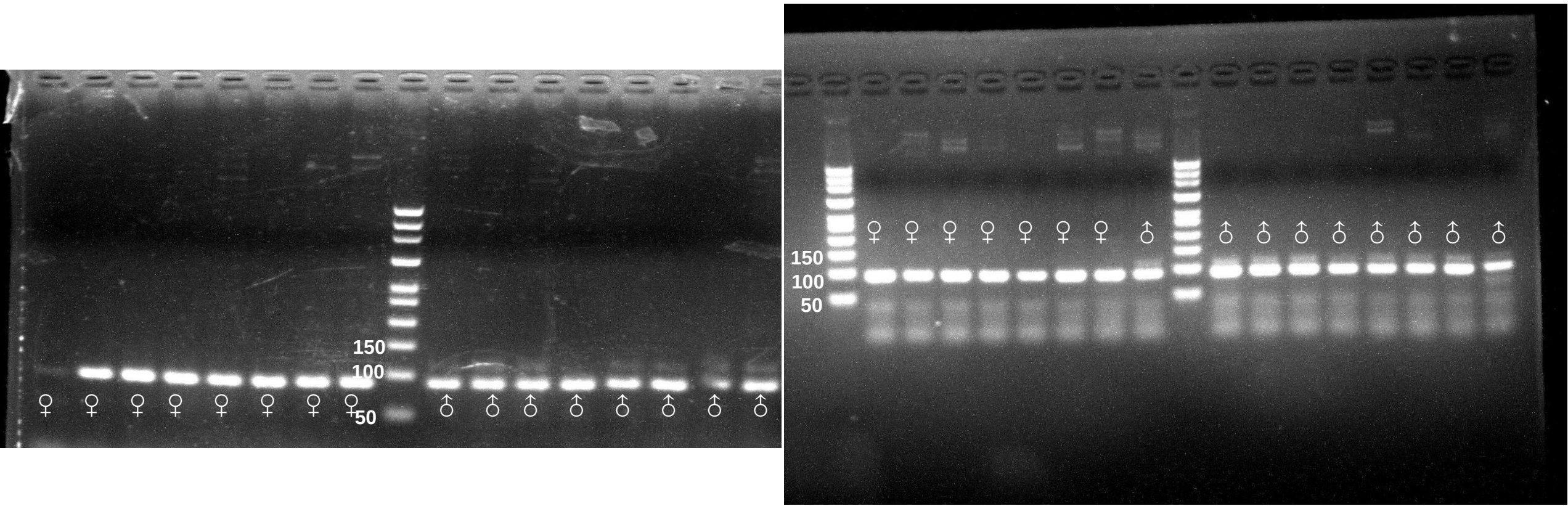
Figure S1. Amplification of 32 genomic DNAs from A. arguta plants by the maker aC36306. For male A. arguta samples, two bands are expected to be present at the gel. ♀ = female, ♂ = male.
