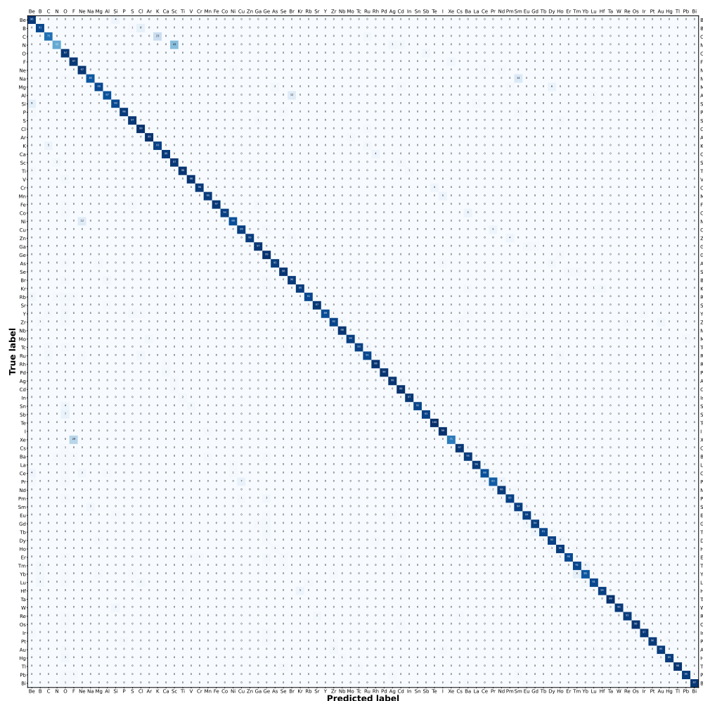
Figure 8. Confusion matrix of the 2xViT+3xU-Net ensemble
