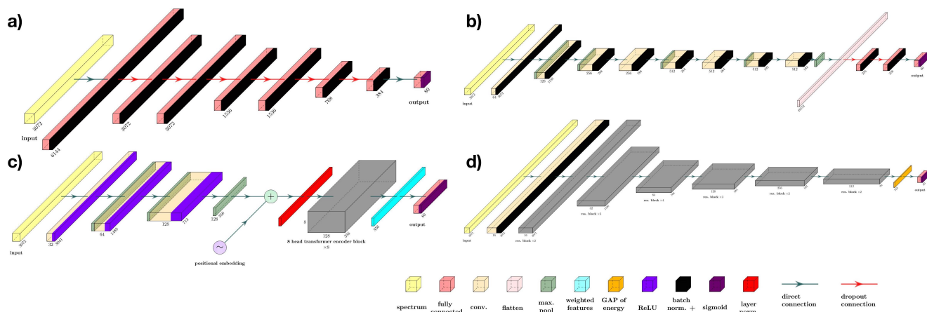
Figure 9. Remaining schematics of compared neural network architectures. a) Multilayer perceptron b) Convolutional neural network c) Compact convolutional transformer d) Residual neural network
