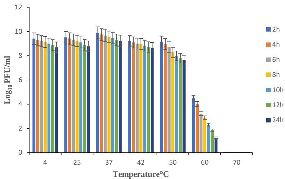
Supplementary Fig. 7. The effects of different temperatures (4 to 70 °C) on the stability of the vB_PaS-HSN4 phage. The results show the mean of three experiments. Bars: standard deviation.
