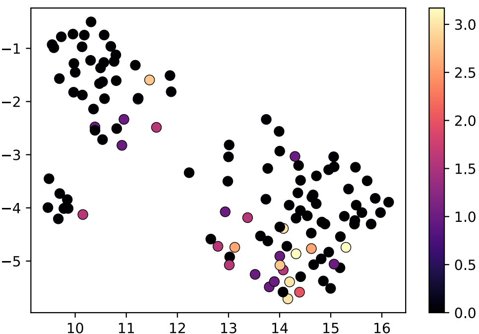
fgfrB (Smp_157300)
