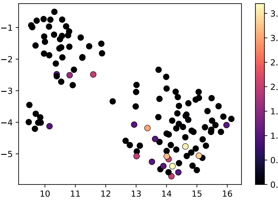
p53 (Smp_139530)
