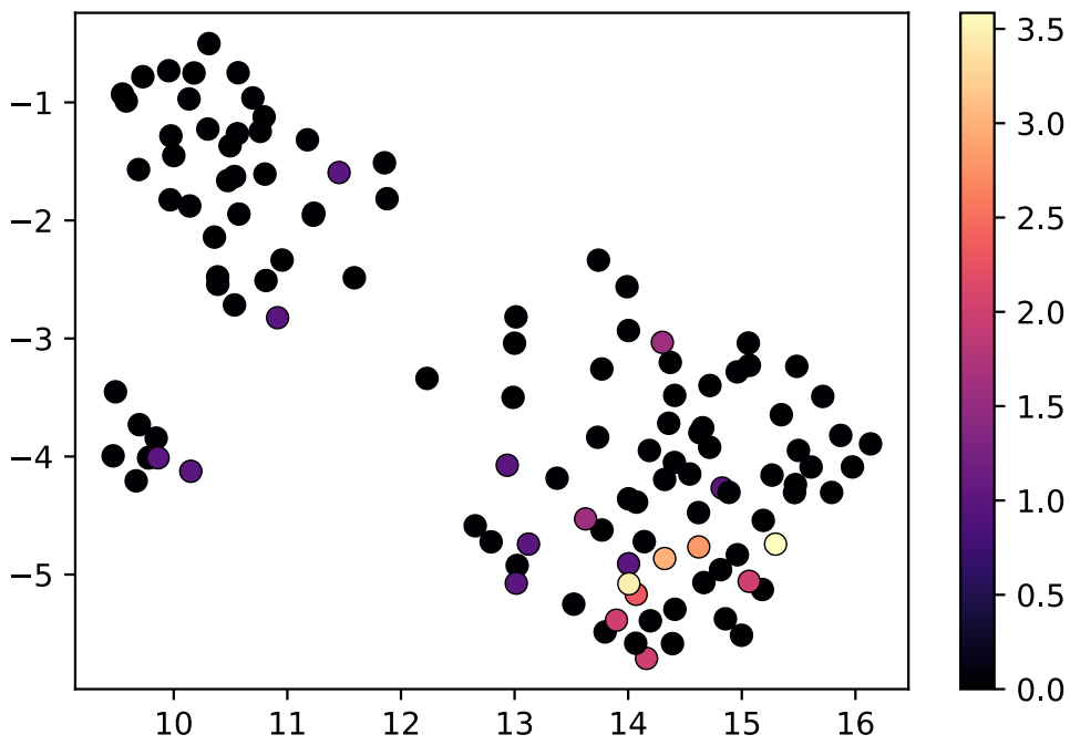
hes1 (Smp_024860)
