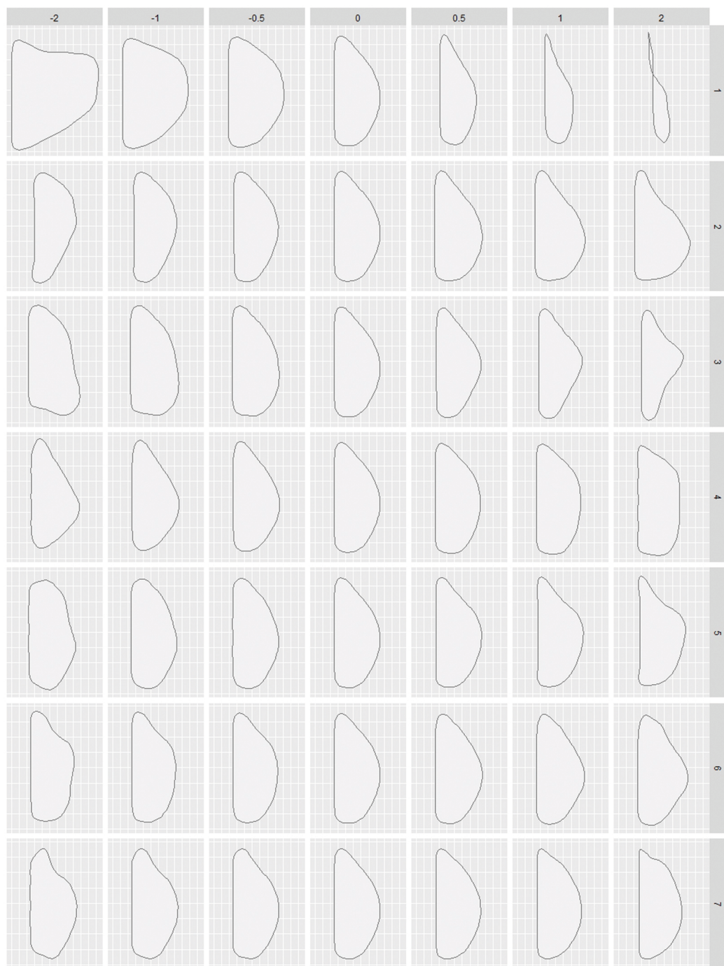
Supplementary Figure S1: Graphical component loadings of first 17 PCs of PCA on shield outlines.
