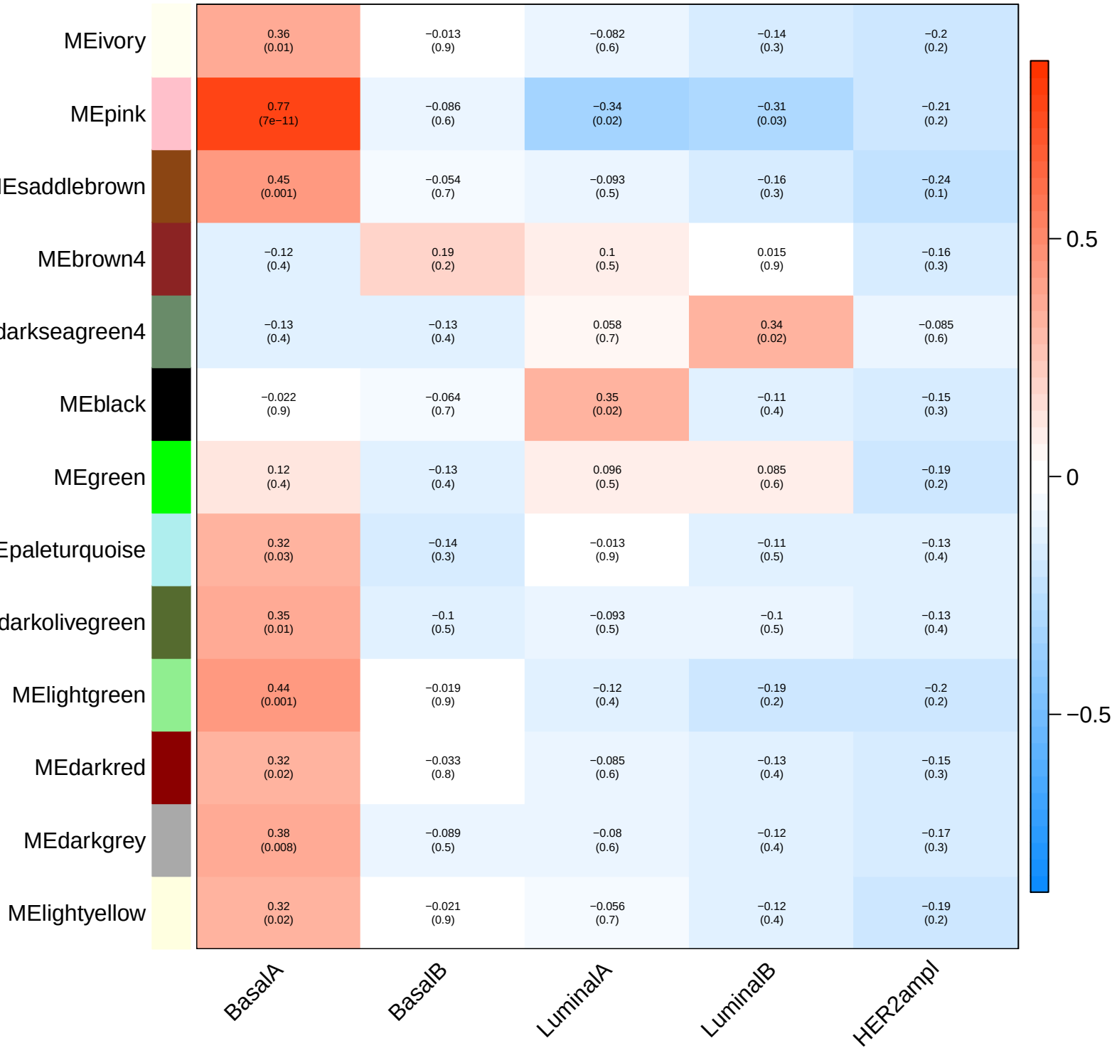
Module–trait relationships(page 2)
