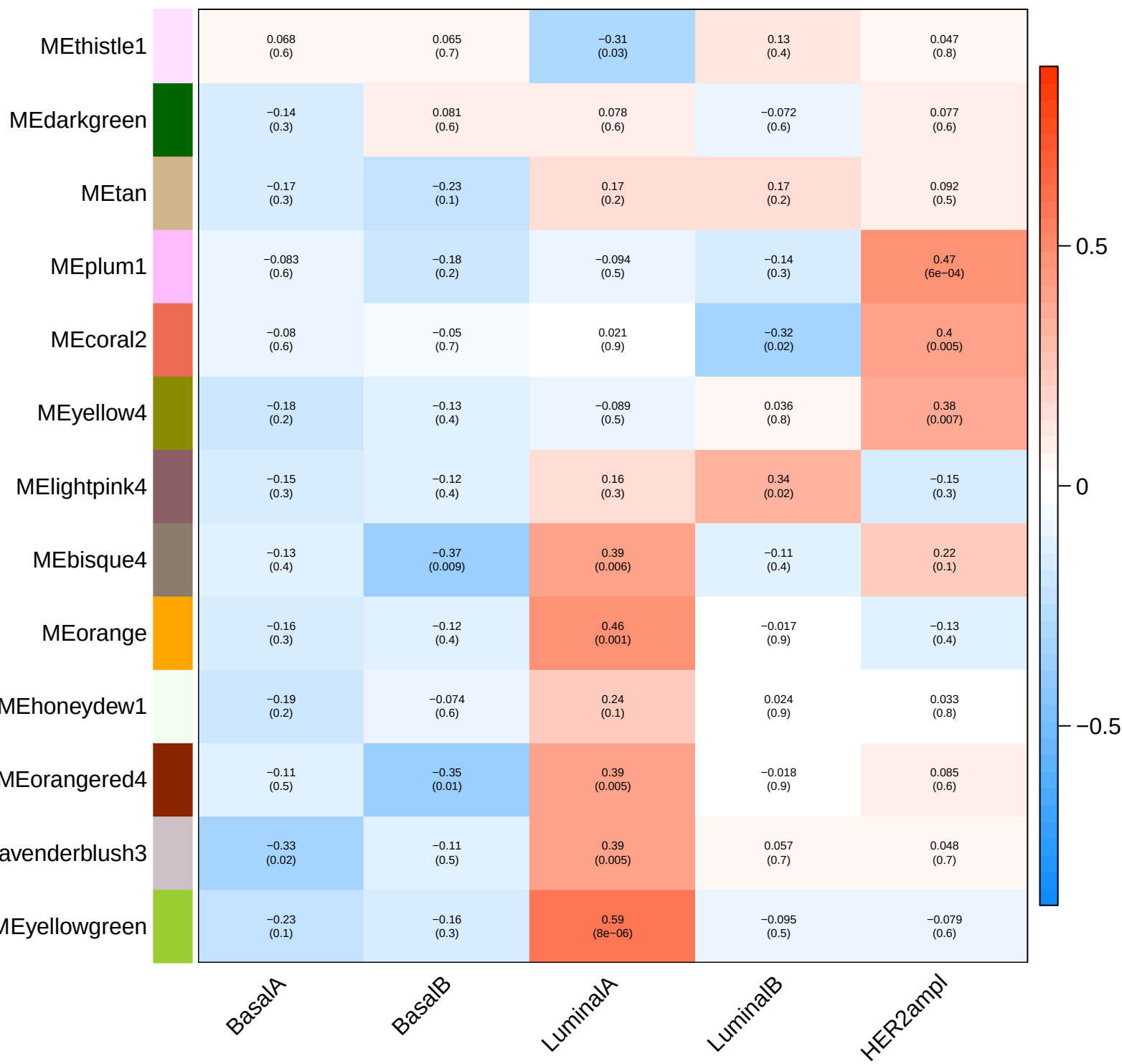
Module–trait relationships(page 4)
