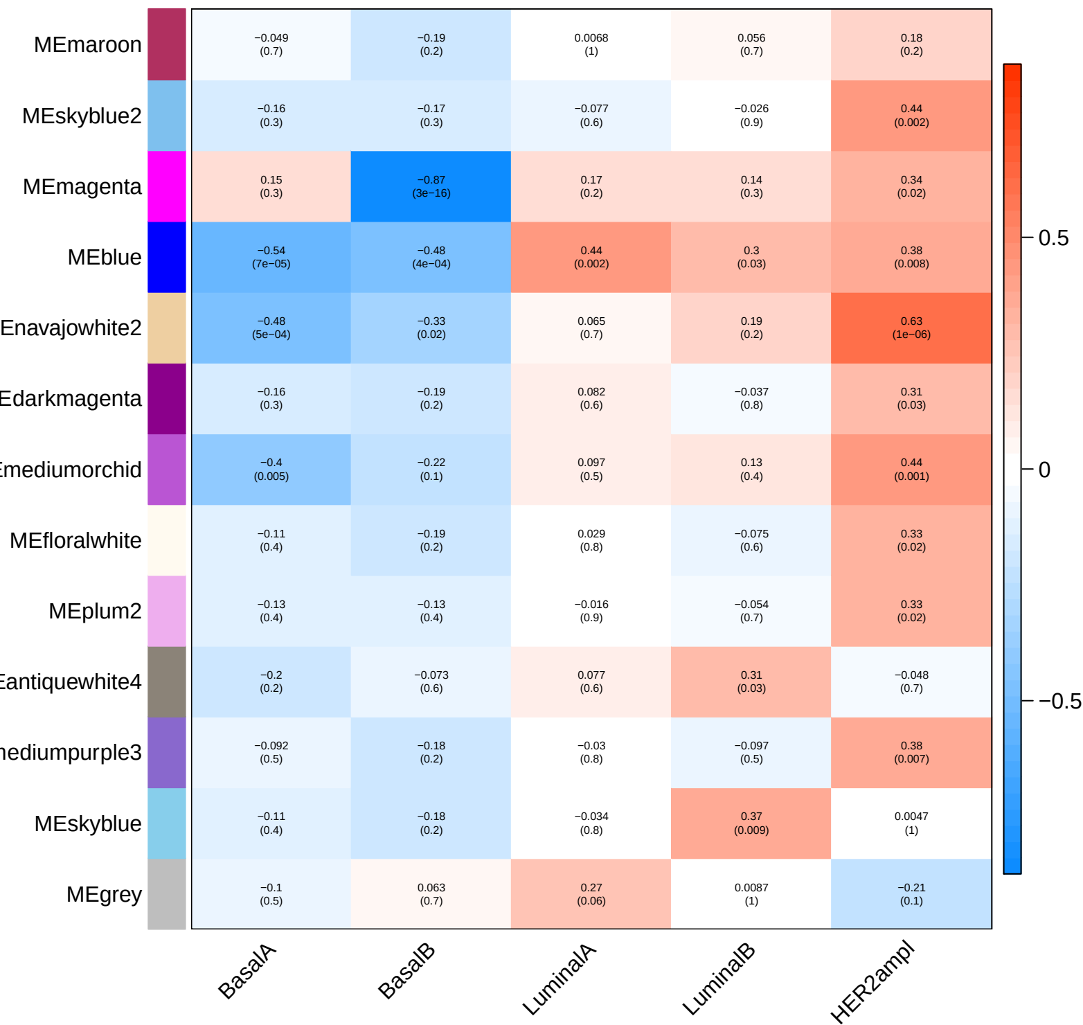
Module–trait relationships(page 5)
