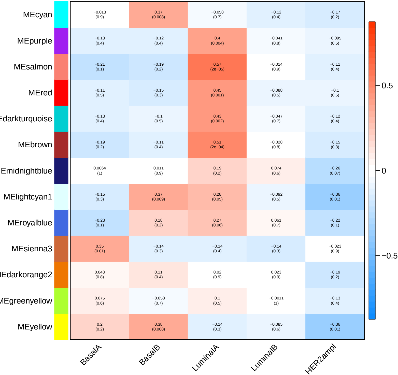
Module–trait relationships(page 3)
