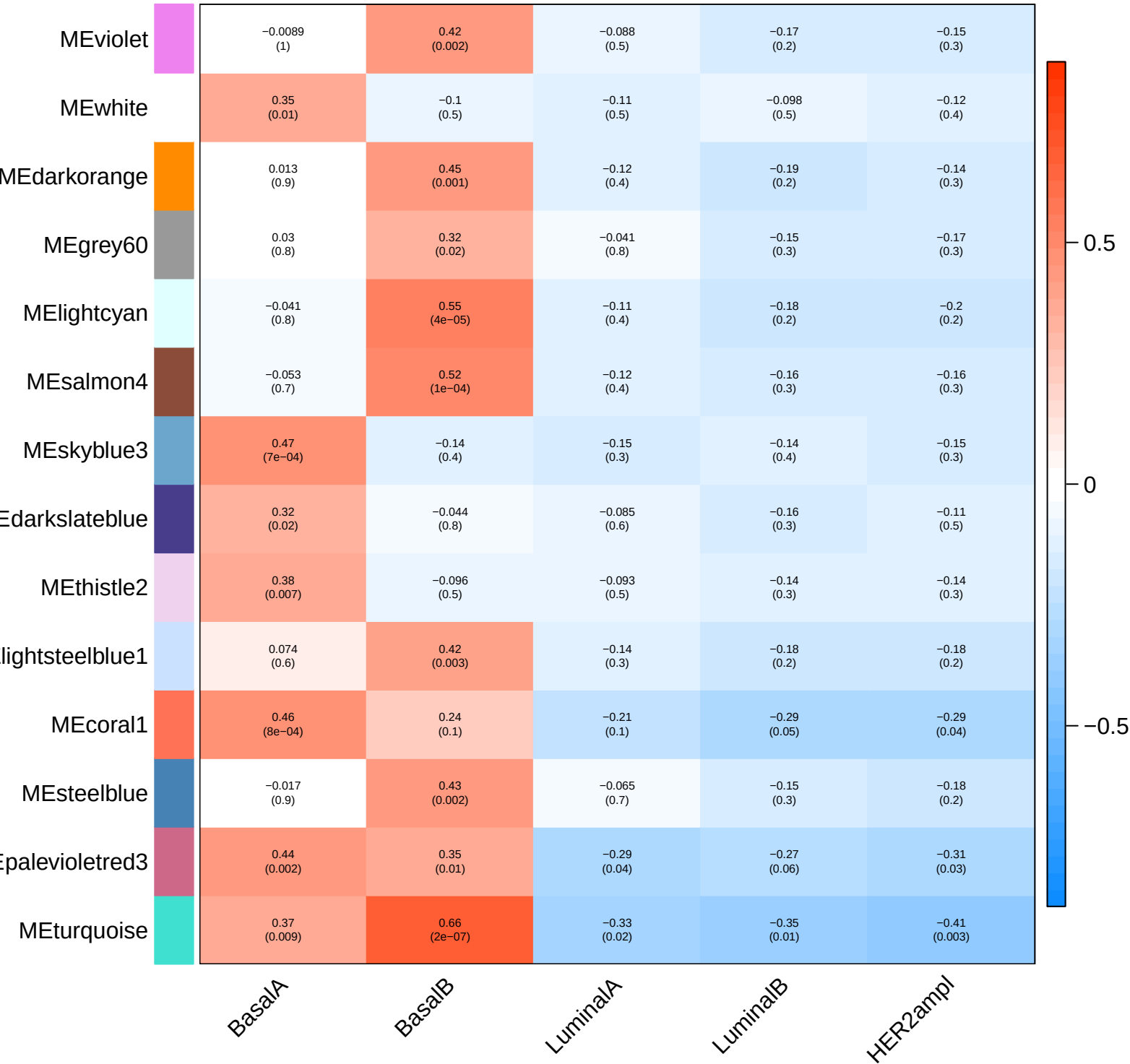
Module–trait relationships(page 1)
