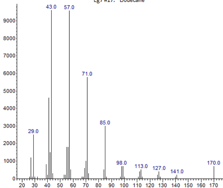
Eg7 #17: Dodecane
