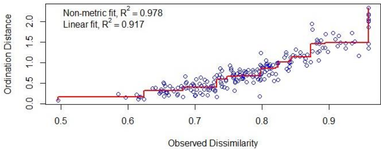
Figure S4. nMDS ordination Stressplot.
