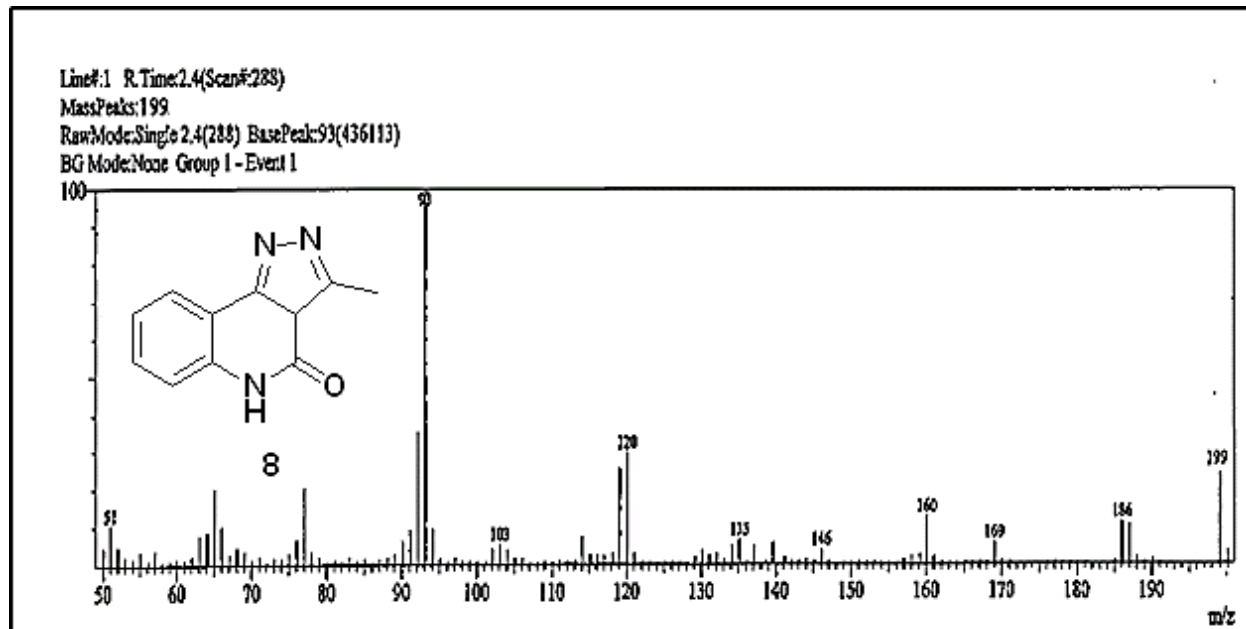
Fig. 14: Mass Spectrum of compound 8
