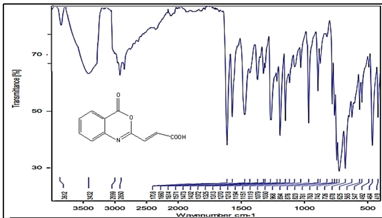
Fig. 15: IR Spectrum of compound 11
