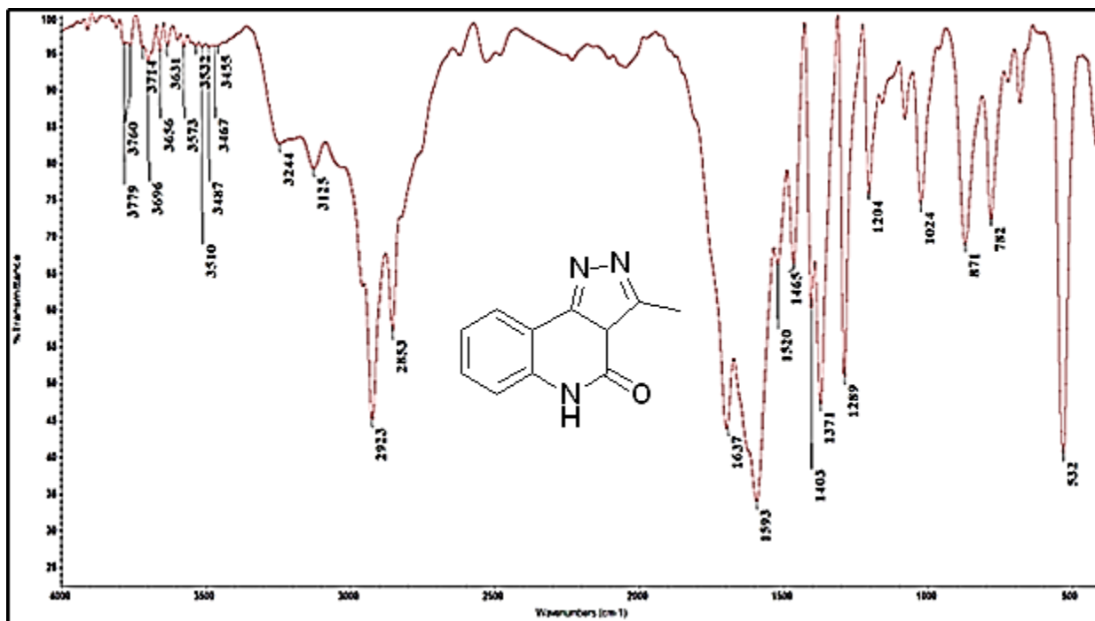
Fig. 10: IR Spectrum of compound 8
