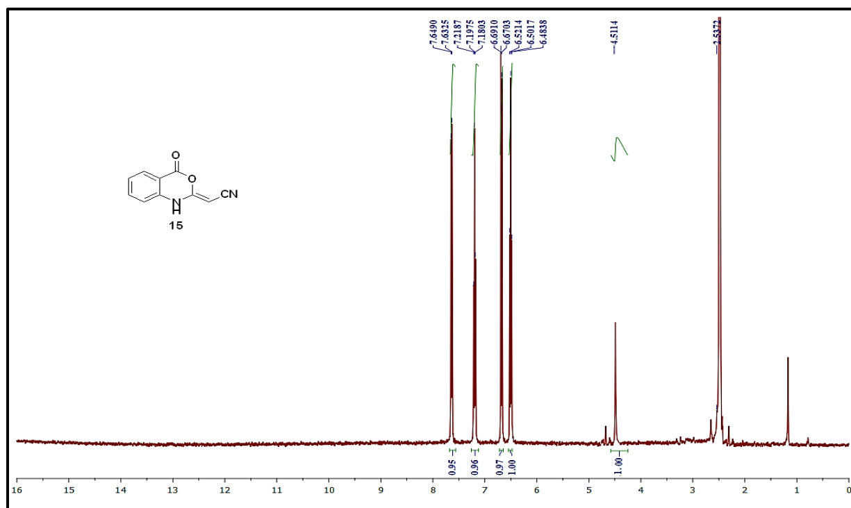
Fig. 25: 1 H-NMR Spectrum (D 2 O) of compound 15
