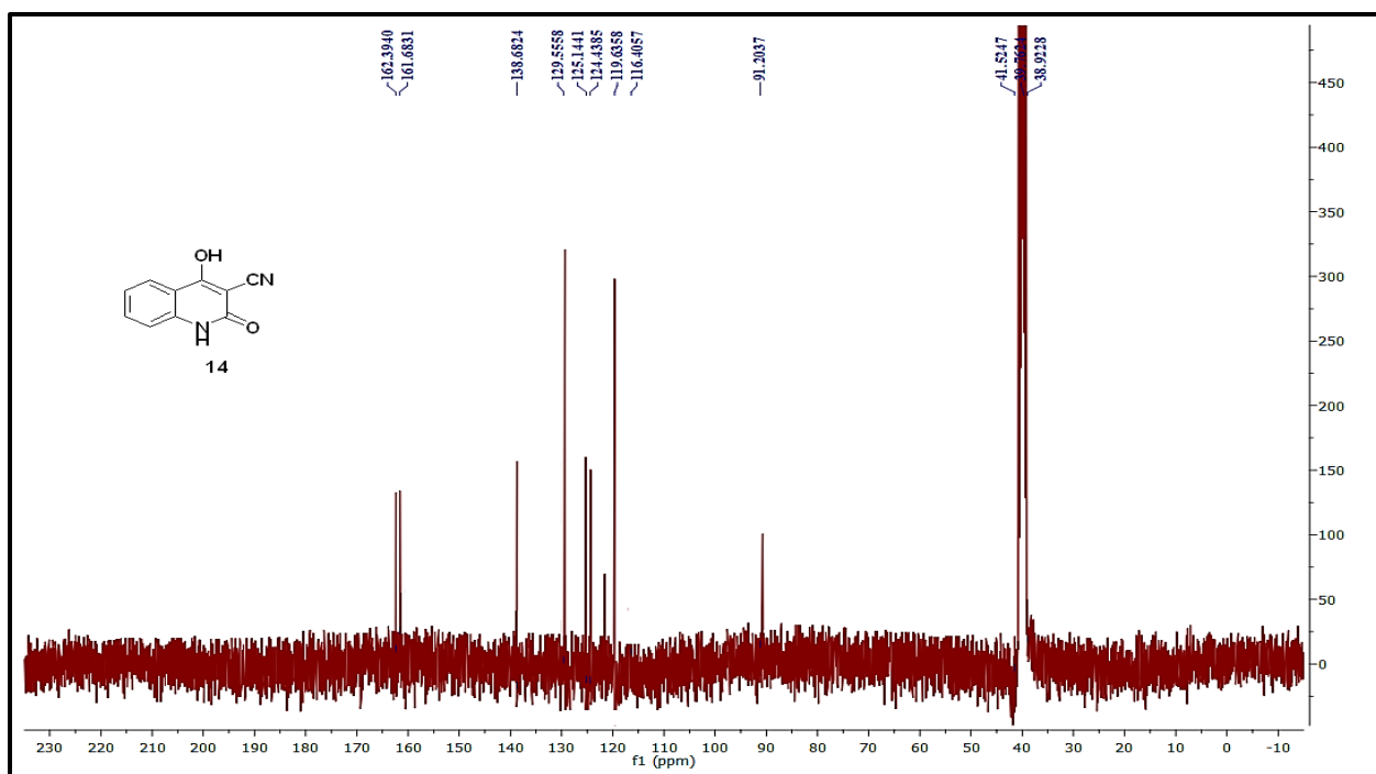
Fig. 21: 13 C-NMR Spectrum of compound 14
