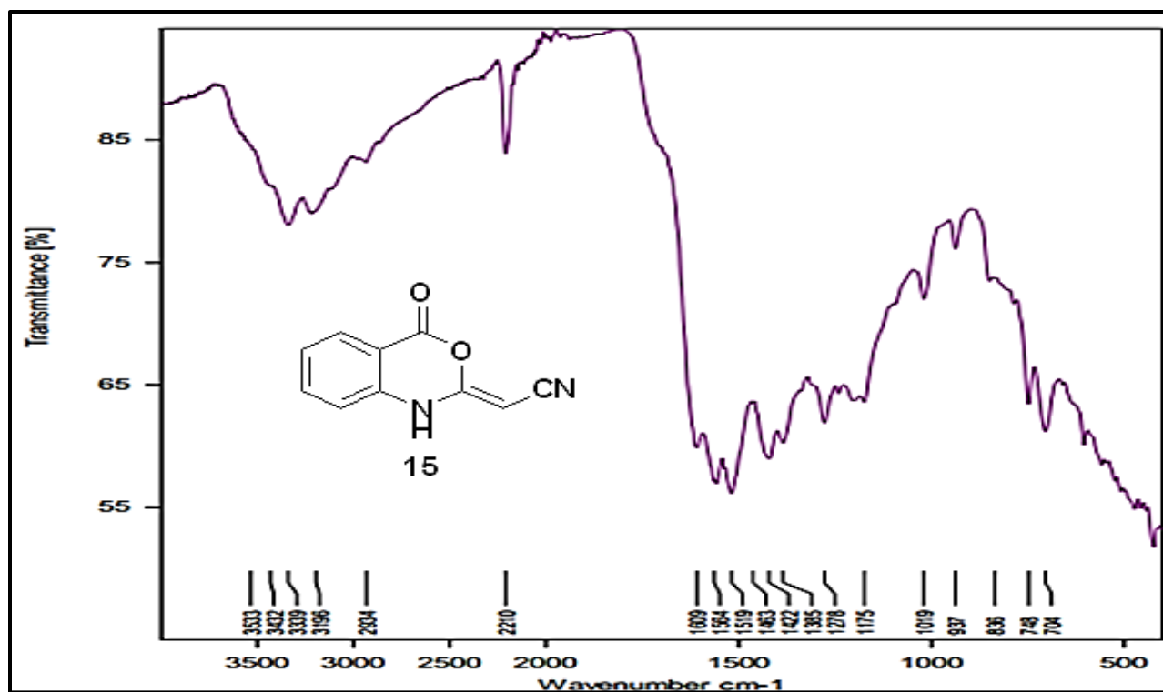
Fig. 23: IR Spectrum of compound 15
