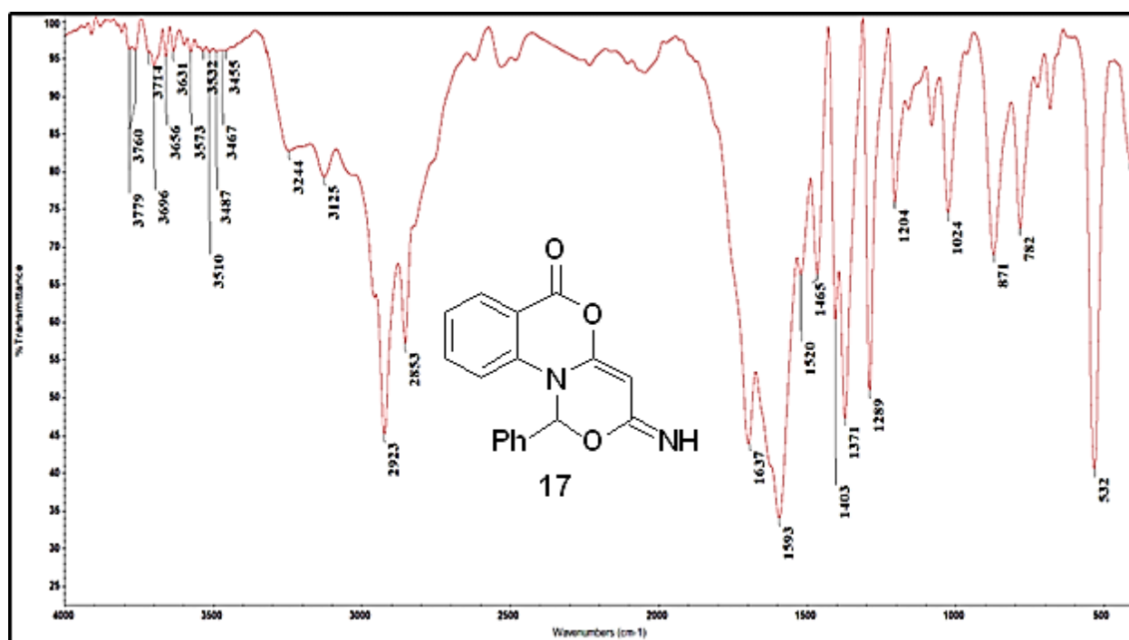
Fig. 28: IR Spectrum of compound 17
