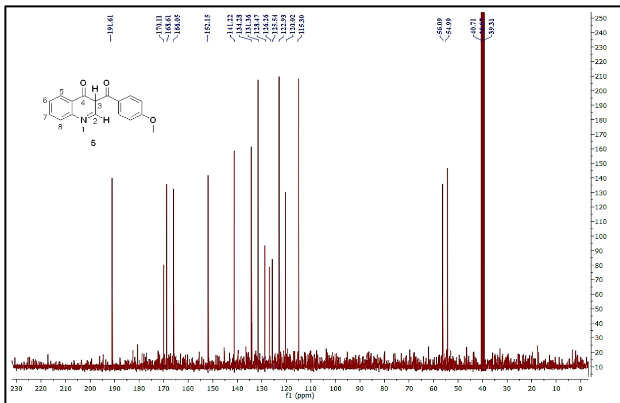
Fig. 3: ^{13}\text{C} -NMR Spectrum of compound 5
