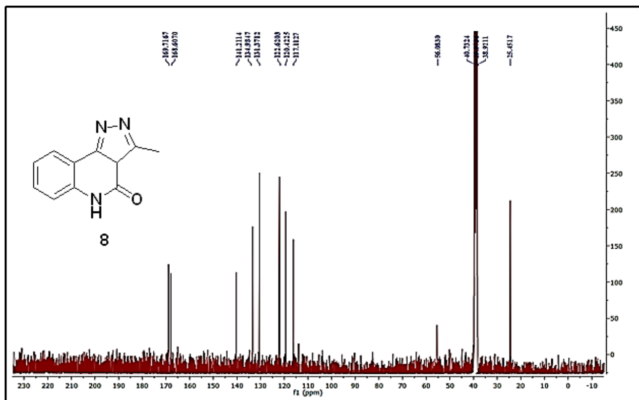
Fig. 13: 13 C-NMR Spectrum of compound 8
