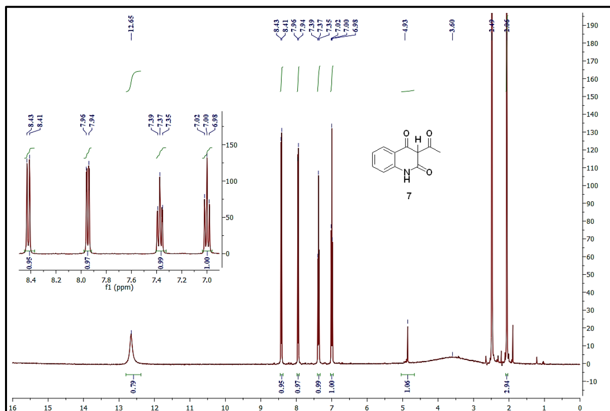
Fig. 6: 1 H-NMR Spectrum of compound 7
