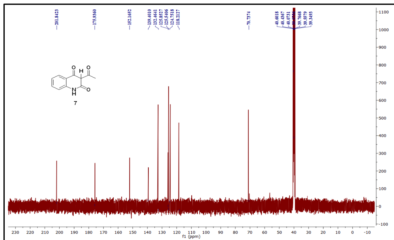
Fig. 8: 13 C-NMR Spectrum of compound 7
