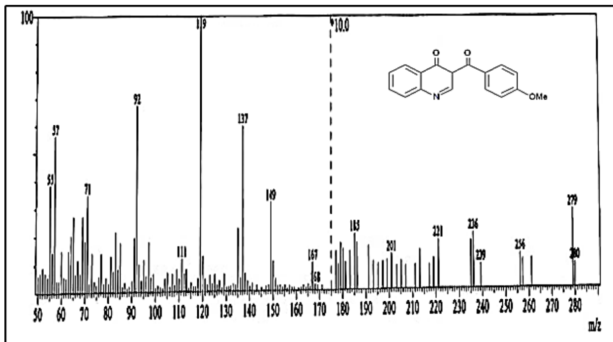
Fig. 4: Mass Spectrum of compound 5
