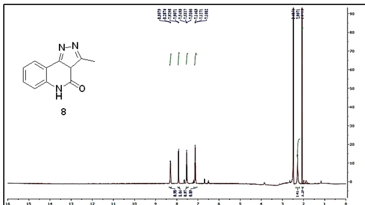
Fig. 12: 1 H-NMR Spectrum (D 2 O) of compound 8
