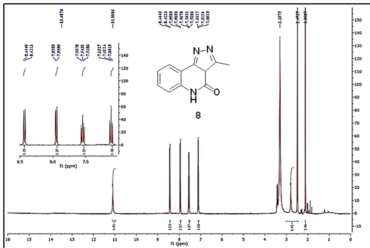
Fig. 11: 1 H-NMR Spectrum of compound 8
