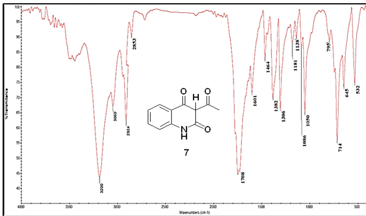
Fig. 5: IR Spectrum of compound 7
