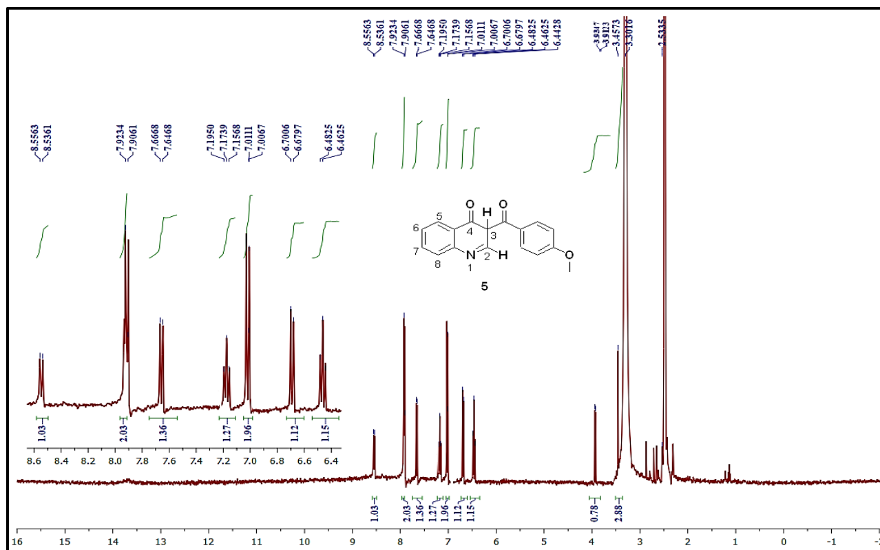
Fig. 2: 1 H-NMR Spectrum of compound 5
