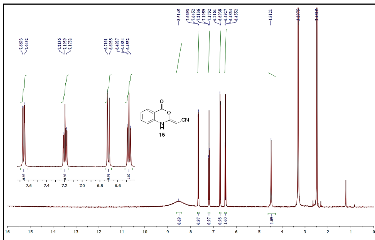
Fig. 24: ^1\text{H-NMR} Spectrum of compound 15
