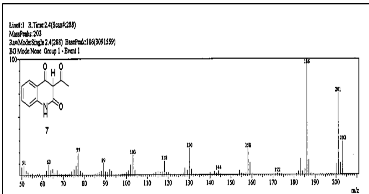
Fig. 9: Mass Spectrum of compound 7
