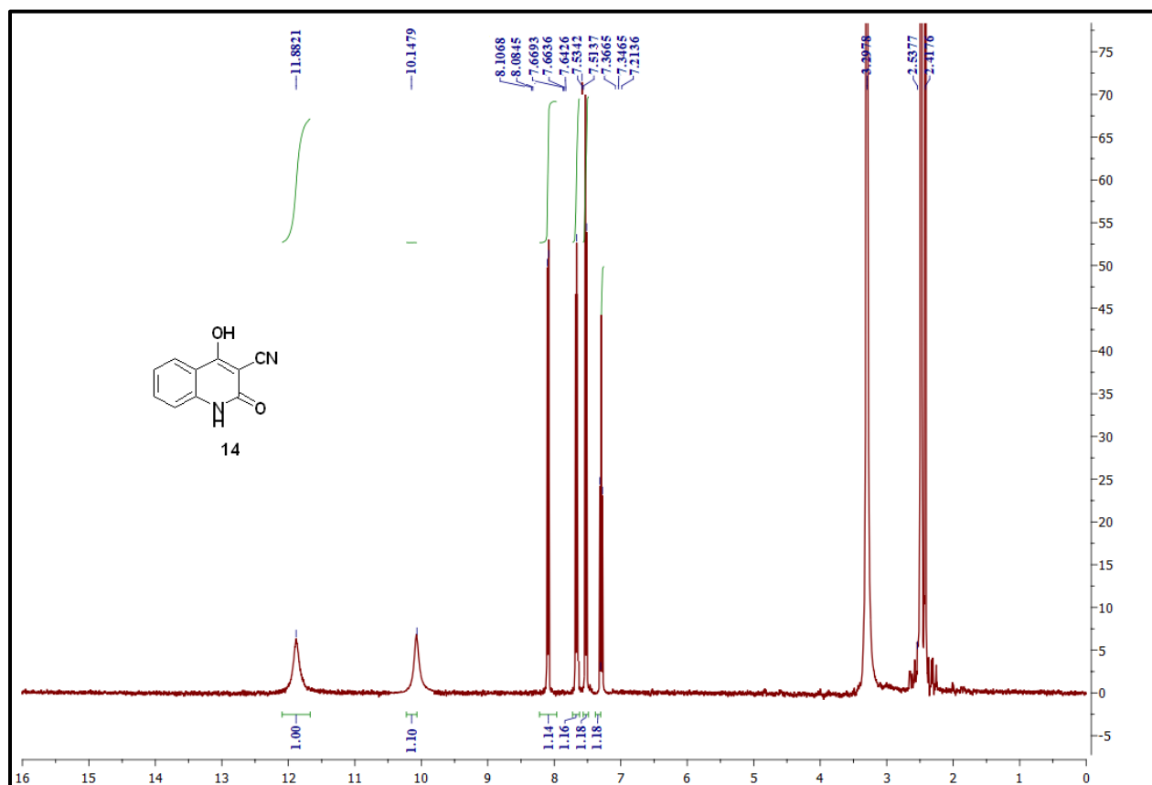
Fig. 20: 1 H-NMR Spectrum of compound 14
