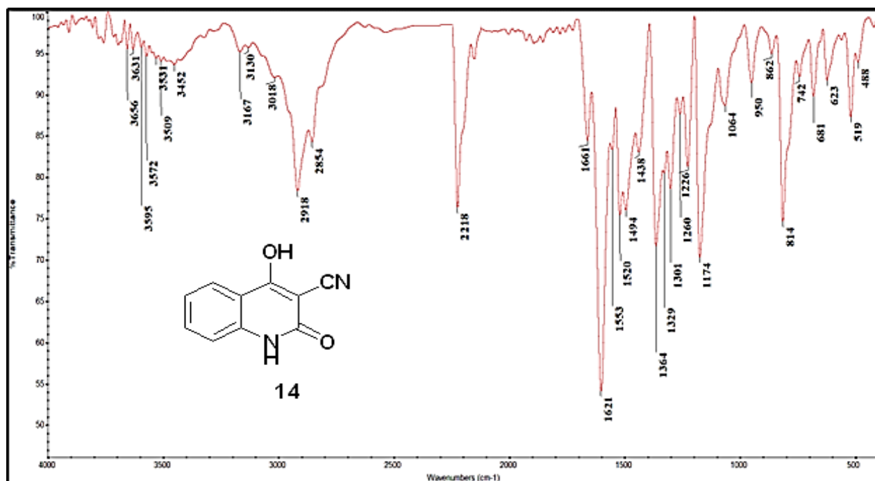
Fig. 19: IR Spectrum of compound 14
