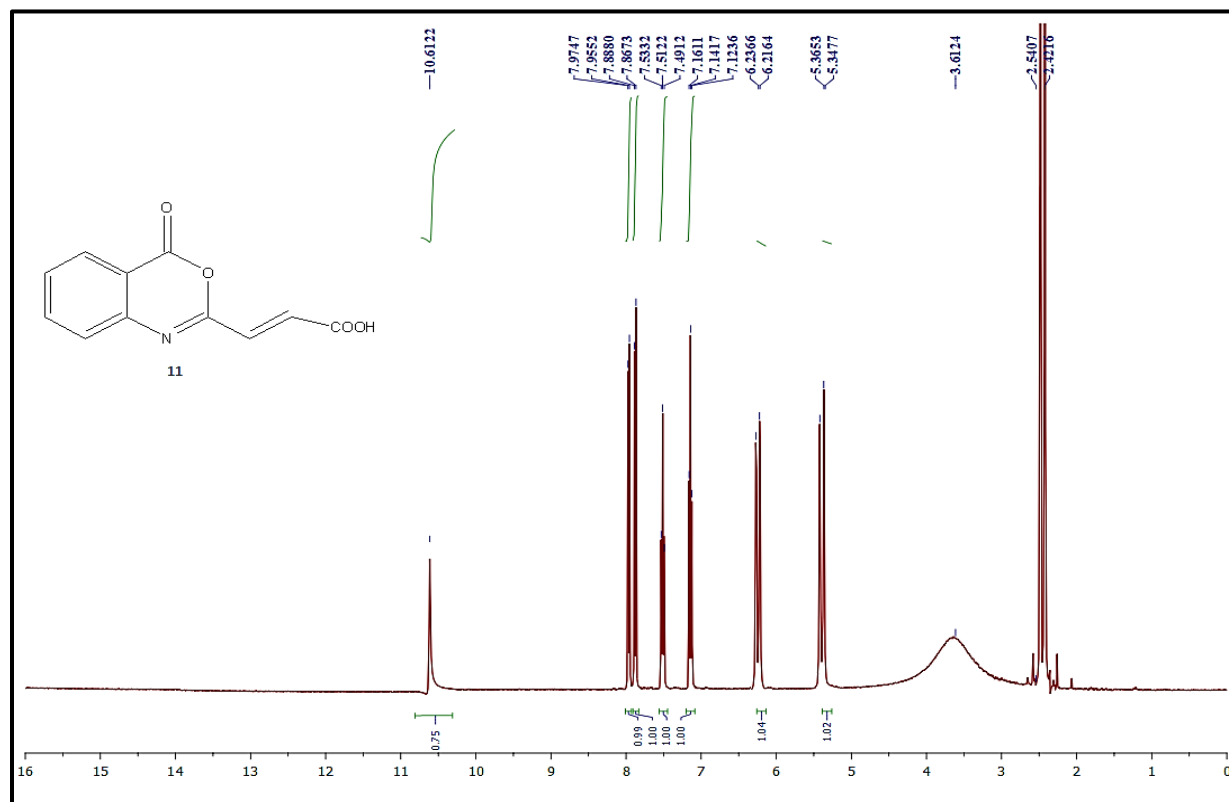
Fig. 16: ^1\text{H} -NMR Spectrum of compound 11
