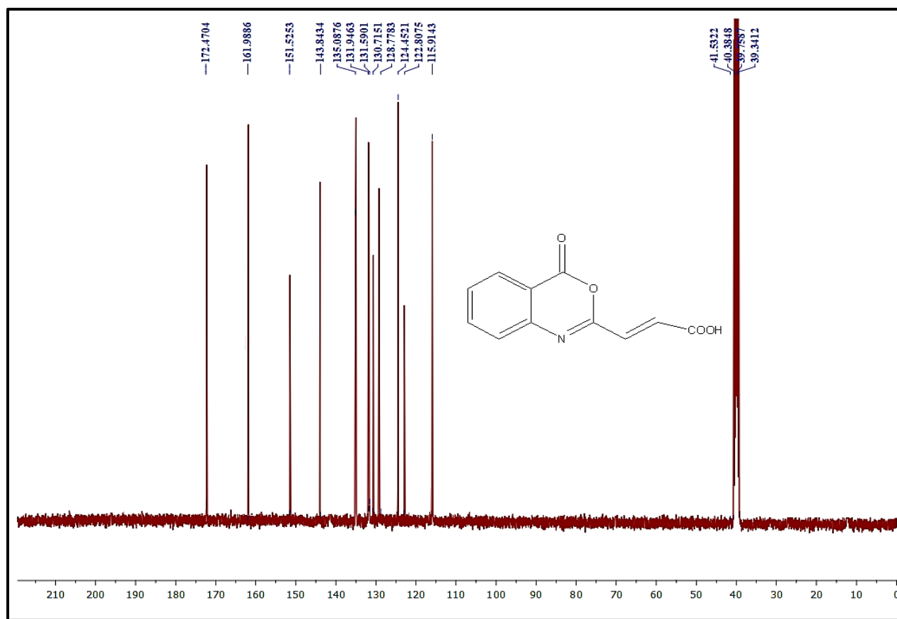
Fig. 17: 13 C-NMR Spectrum of compound 11
