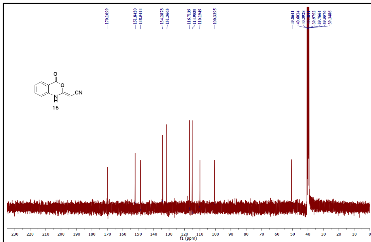
Fig. 26: 13 C-NMR Spectrum of compound 15
