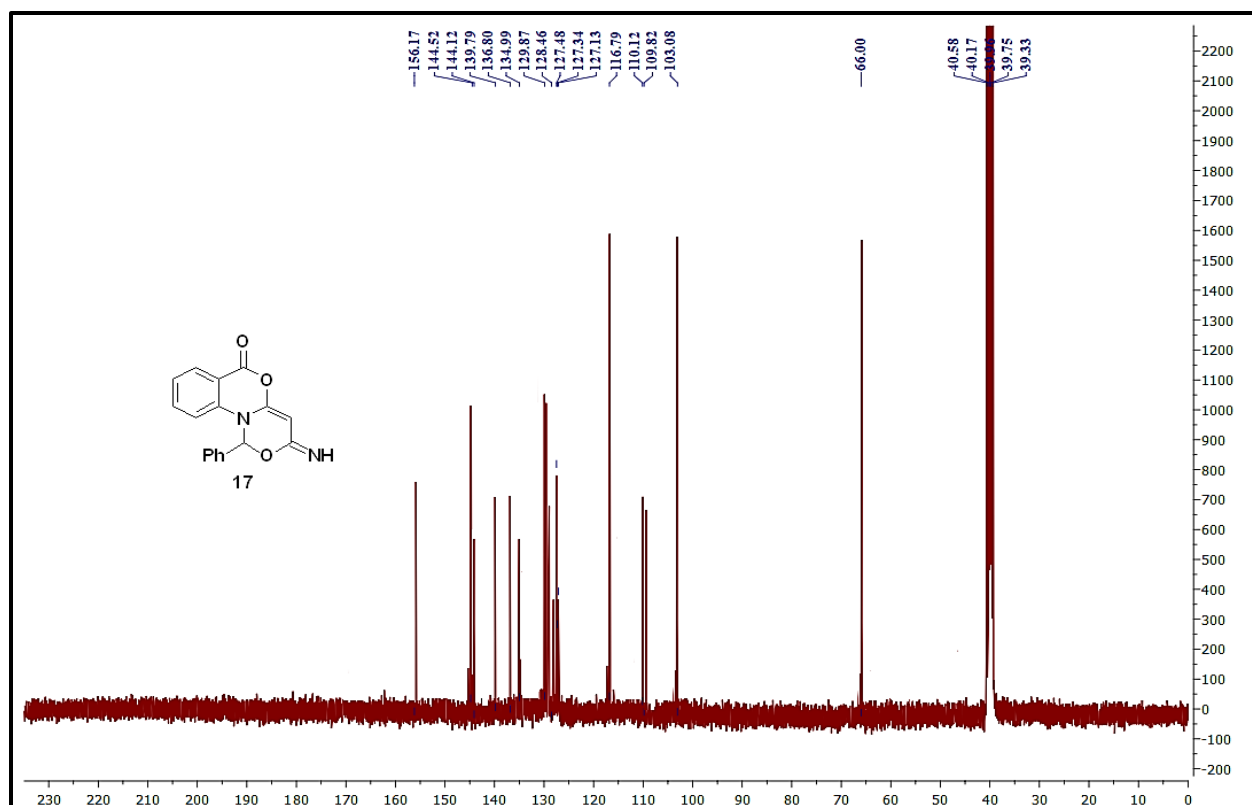
Fig. 31: 13 C-NMR Spectrum of compound 17
