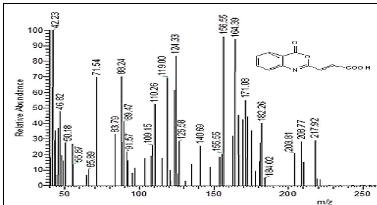
Fig. 18: Mass Spectrum of compound 11
