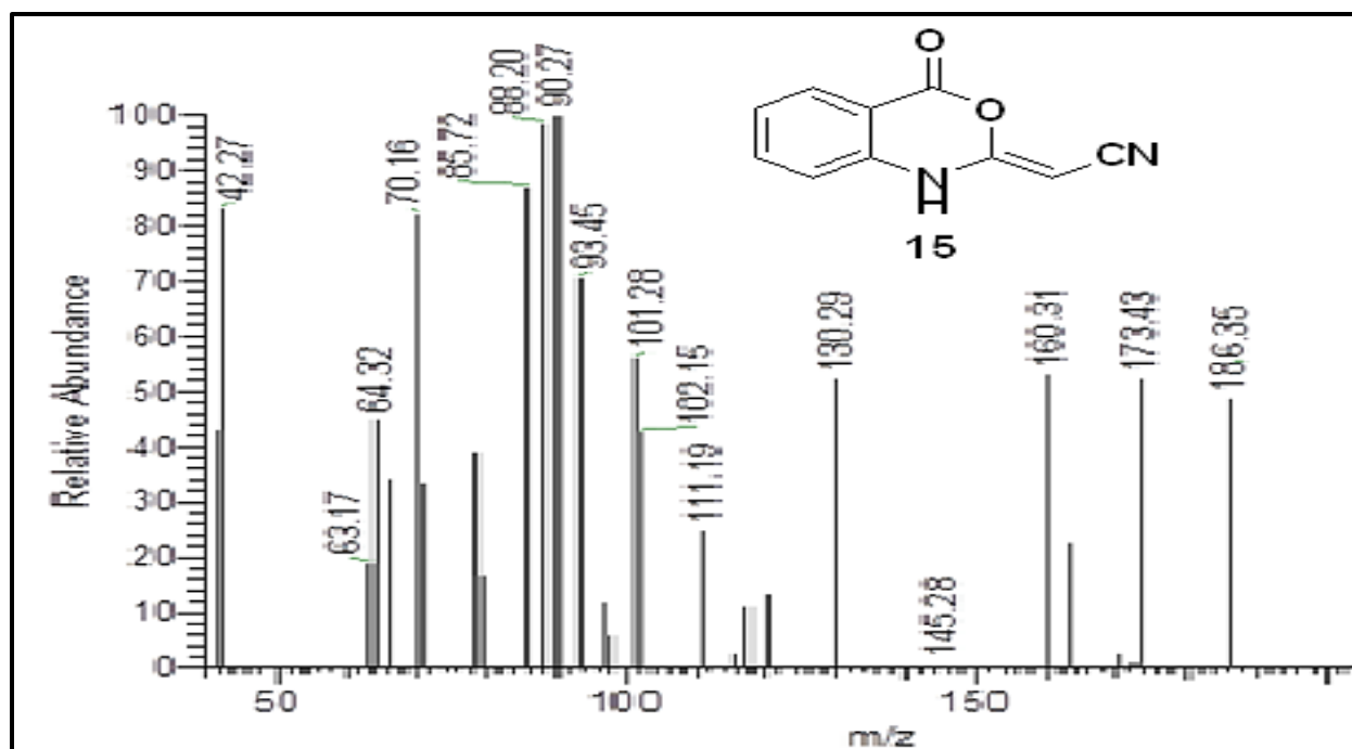
Fig. 27: Mass Spectrum of compound 15
