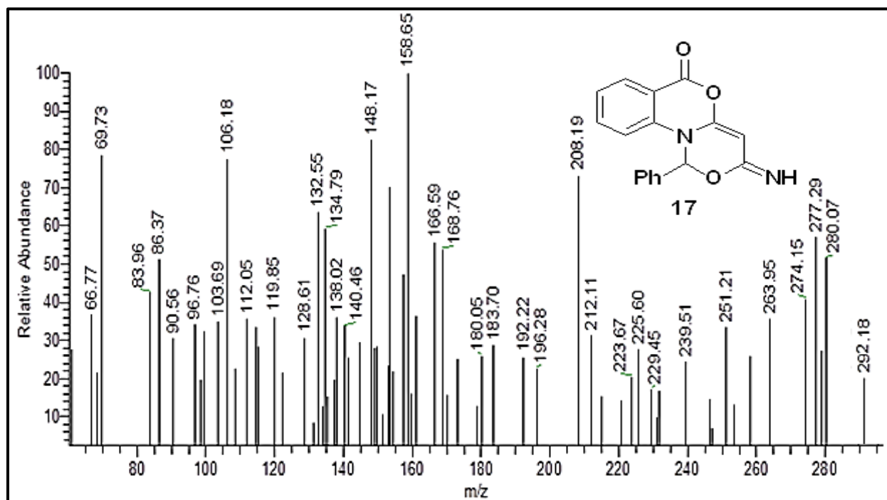
Fig. 32: Mass Spectrum of compound 17
