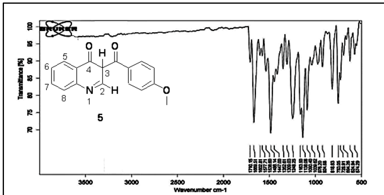
Fig. 1: IR Spectrum of compound 5
