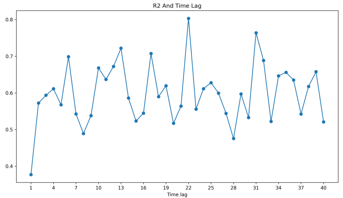
Fig S1 The evaluation metrics MAE, SMAPE, RMSE, and R2 of the XGBoost model vary with changes in the time lag.
