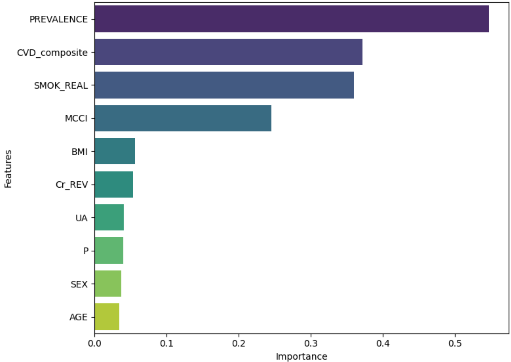
Top 10 Important Features - Lasso Regression
