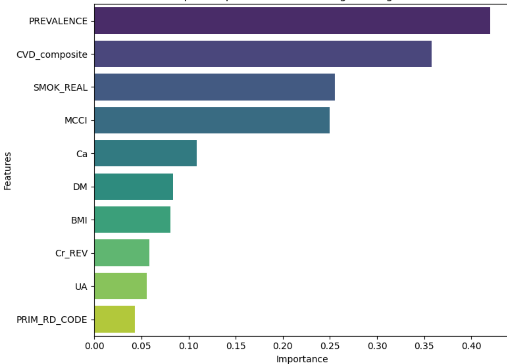
Top 10 Important Features - Logistic Regression
