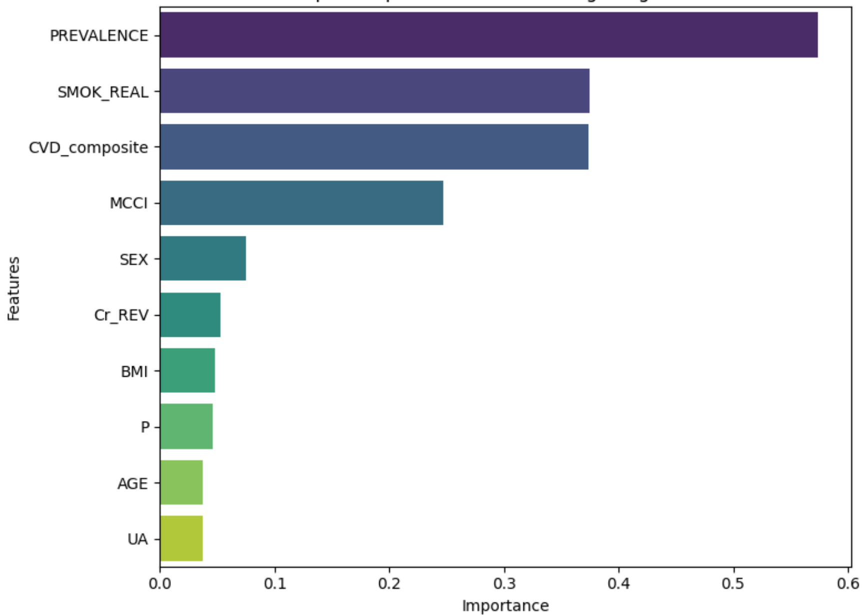
Top 10 Important Features - Ridge Regression
