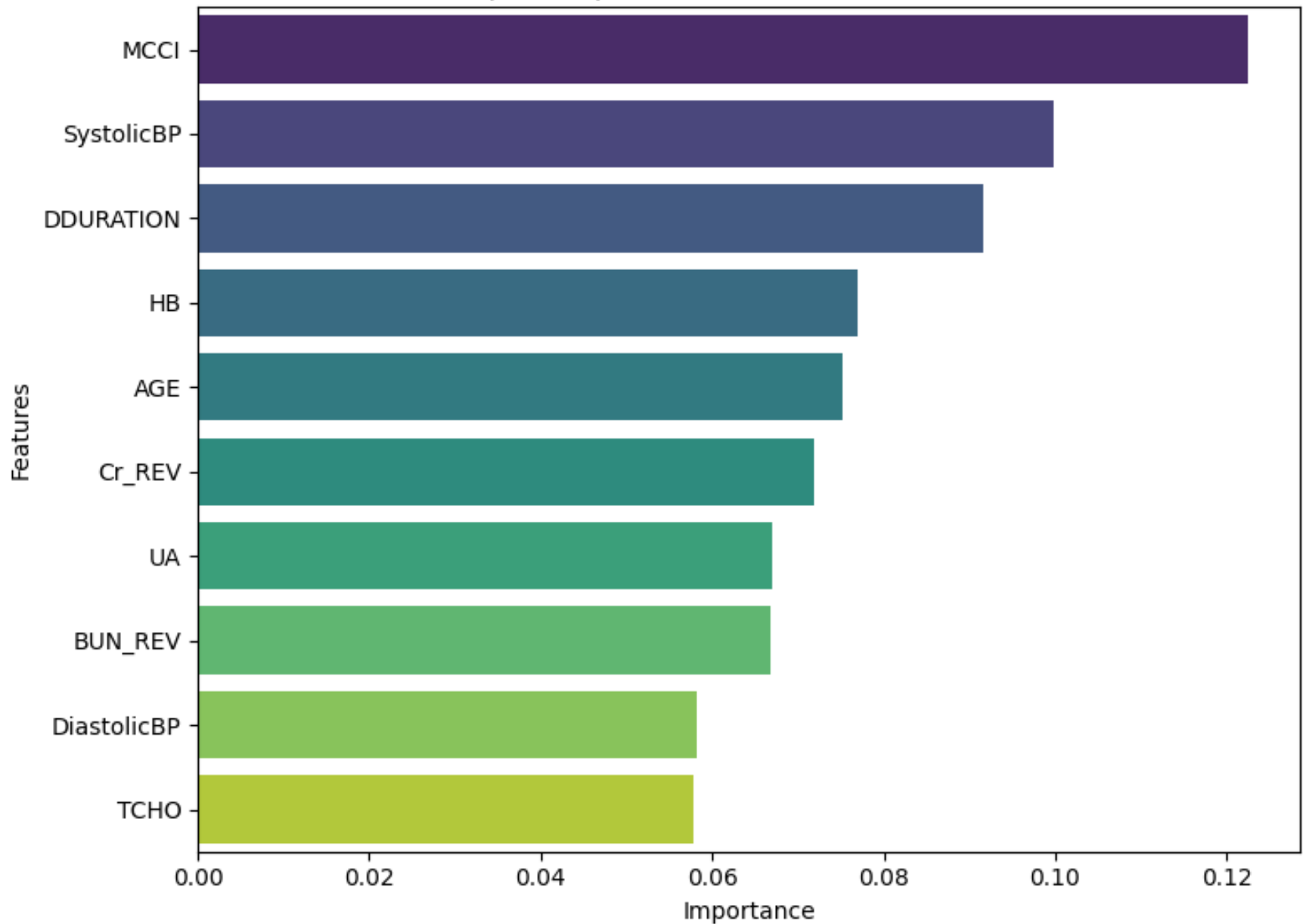
Top 10 Important Features - Decision Tree
