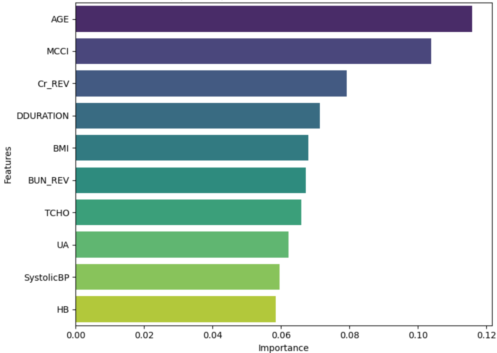
Top 10 Important Features - Random Forest
