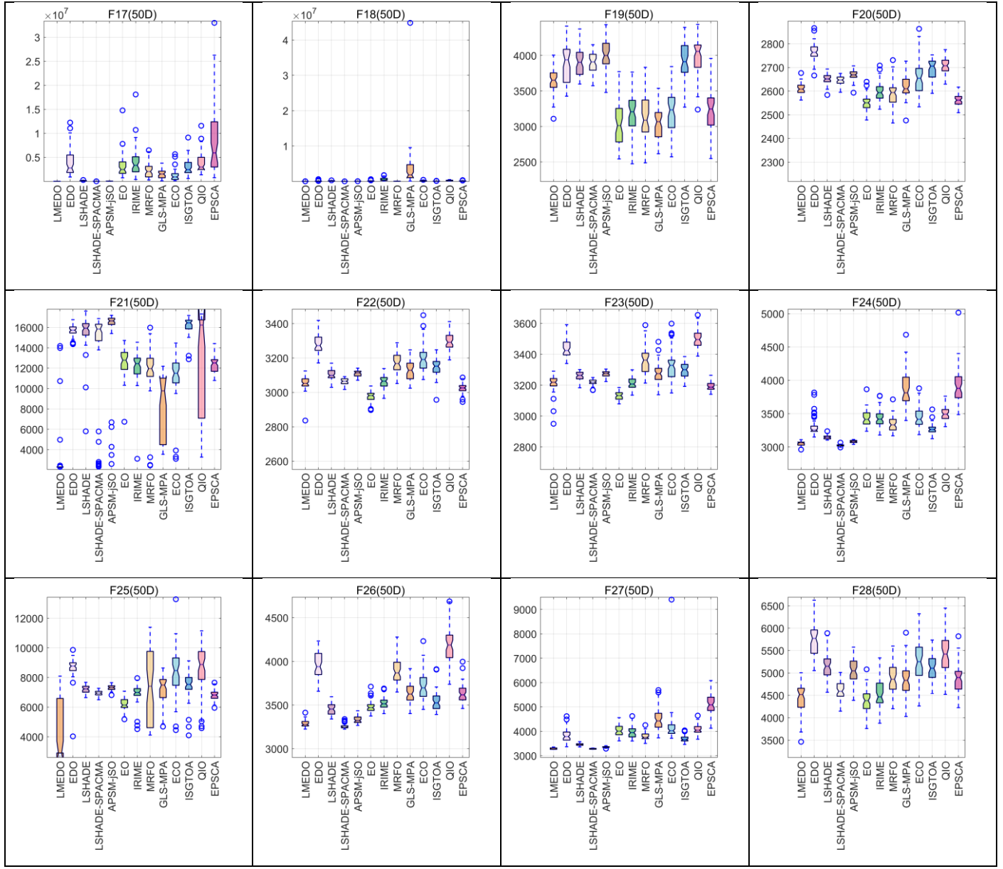
Figure B7. The boxplots of LMEDO and comparison algorithms based on CEC2018 (50D)
