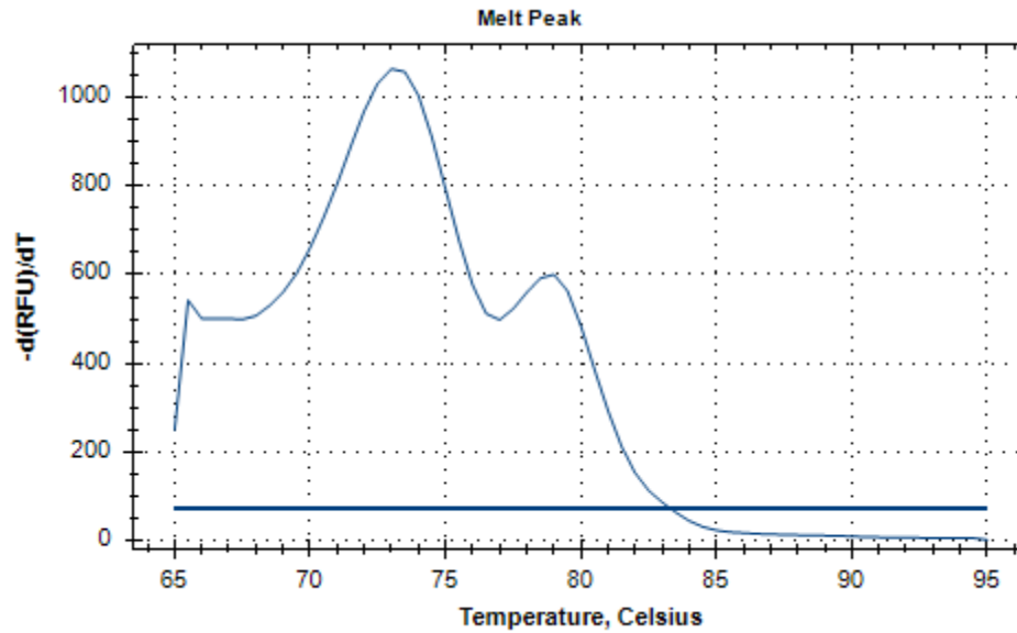
Figure S4. Result of primer specificity analysis on the mouse Prssly gene using the melting curve of the PCR product.
