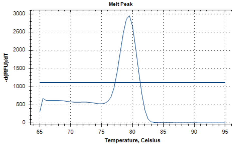
Figure S2. Result of primer specificity analysis for the mouse Gapdh gene using the melting curve of the PCR product.
