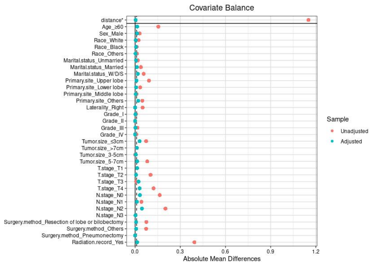
Figure S1 Visualization of PSM to balance baseline features with a caliper of 0.01
