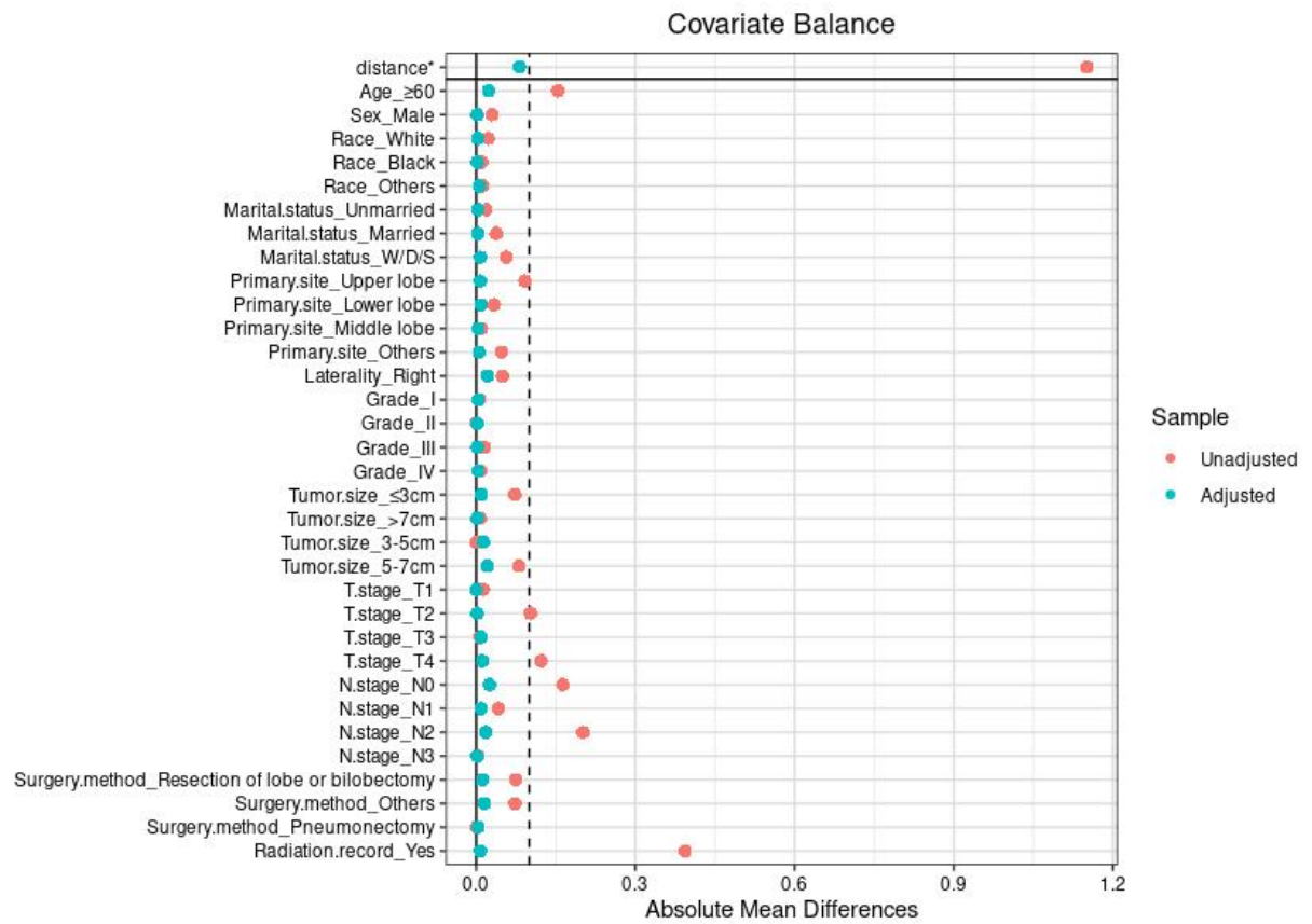
Figure S2 Visualization of PSM to balance baseline features with a caliper of 0.1
