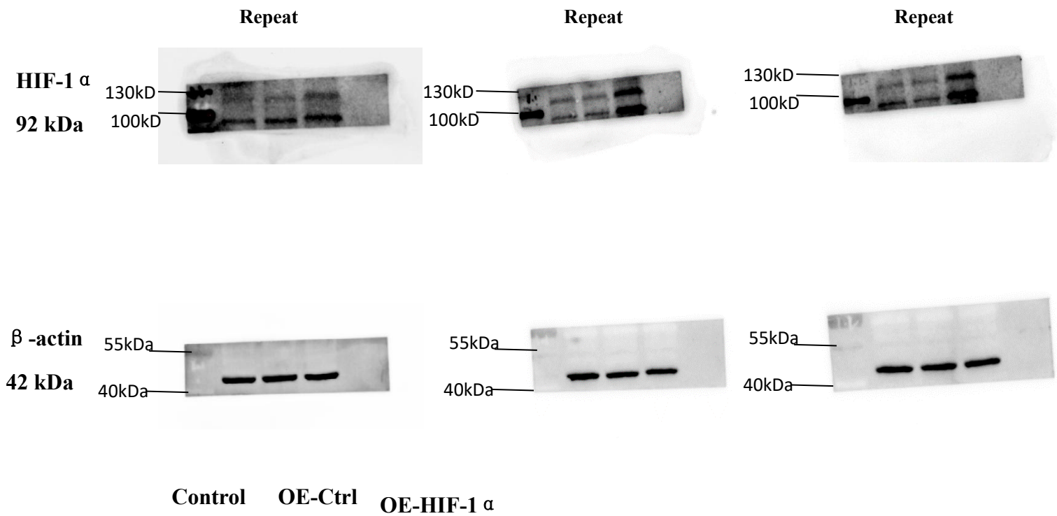
Fig3-A shows the whole blot after cutting membrane at molecular weigh.
