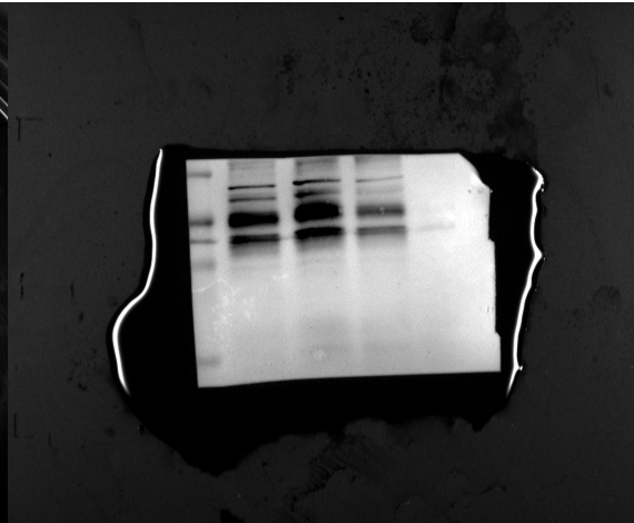
SIRT3-2 he
