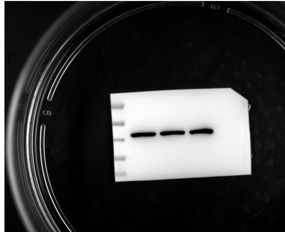
Actin
