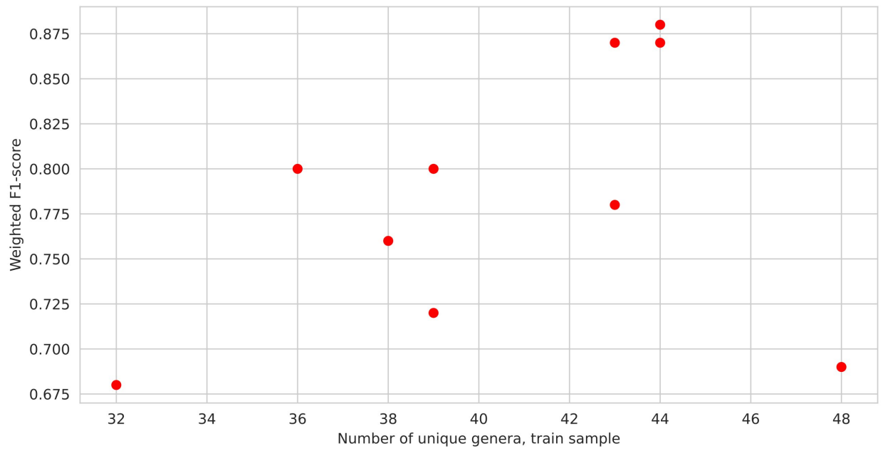
Figure S2. Impact of the number of unique genera in training sample on the weighted F1-score. F1-scores are shown for the top-performing model (SVC trained on nucleotide 4-mers) in ten independent realizations of non-overlapping genera train-test split.
