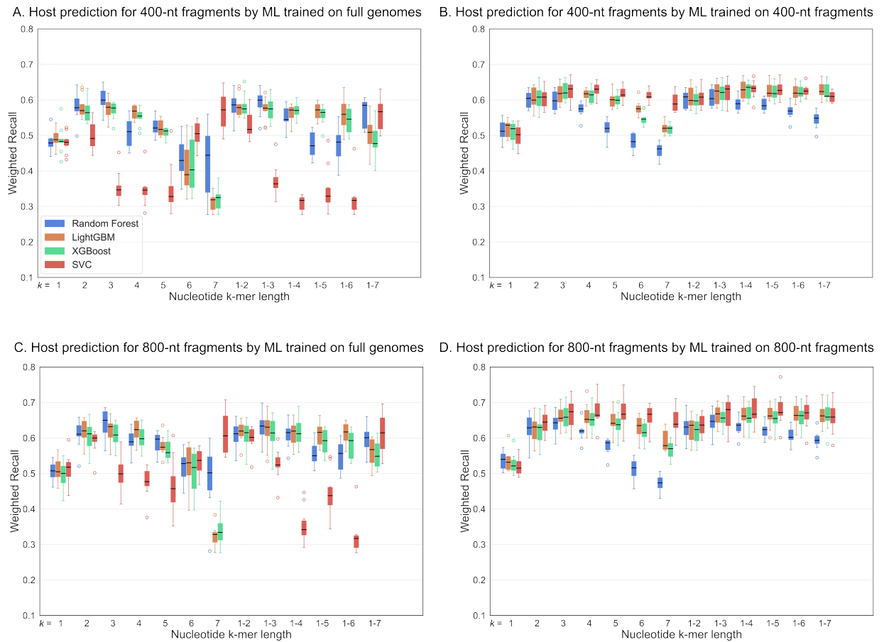
Figure S7. Weighted recall of models tested to predict virus hosts on fragments datasets: classifier trained on full genomes and tested on 400-nt fragments (A); classifier trained and tested on the same length 400-nt fragments (B); classifier trained on full genomes and tested on 800-nt fragments (C); classifier trained and tested on the same length 800-nt fragments (D). Boxplots indicate the distribution of weighted F1-scores for ten train-test split replicates. The models trained in this study: RF – blue, LGBM – orange, XGB – green, and SVC – red).
