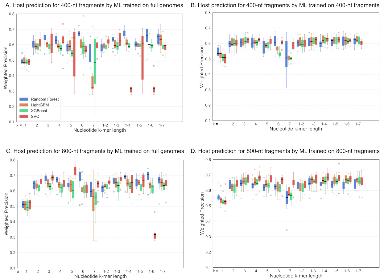
Figure S6. Weighted precision of models tested to predict virus hosts on fragments
