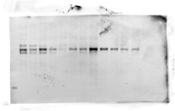
CYP17A1
