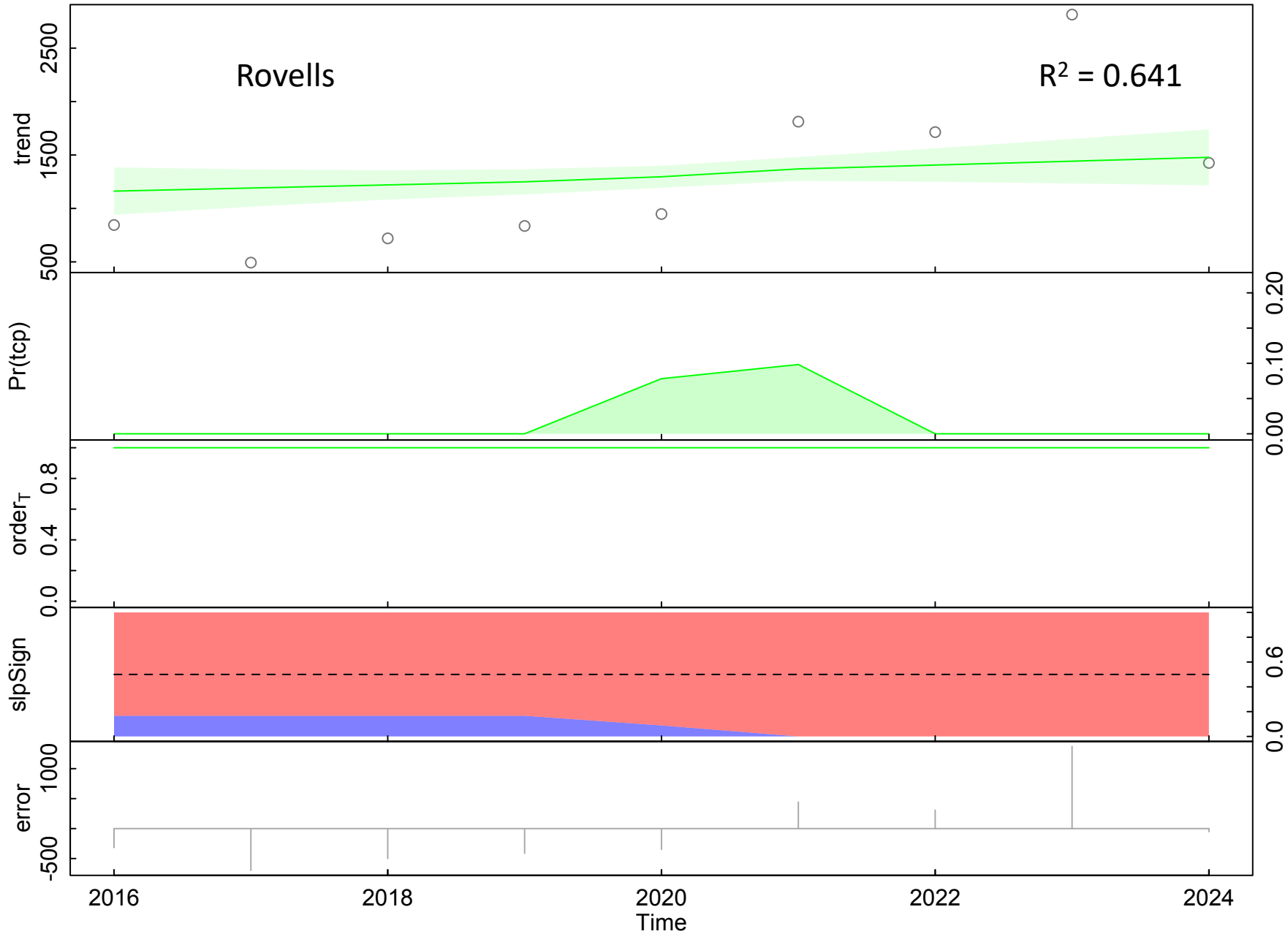
BEAST decomposition and changepoint detection
