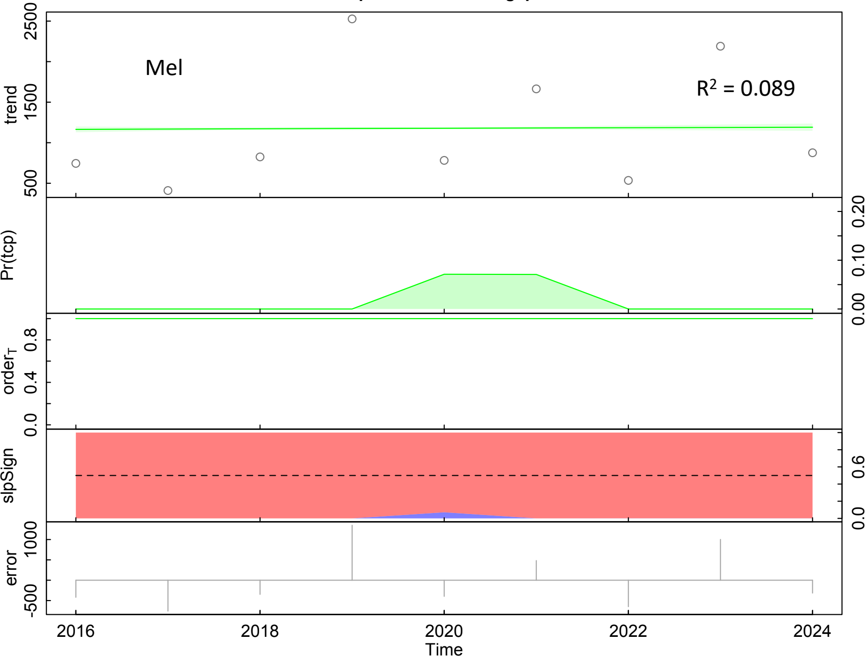
BEAST decomposition and changepoint detection
