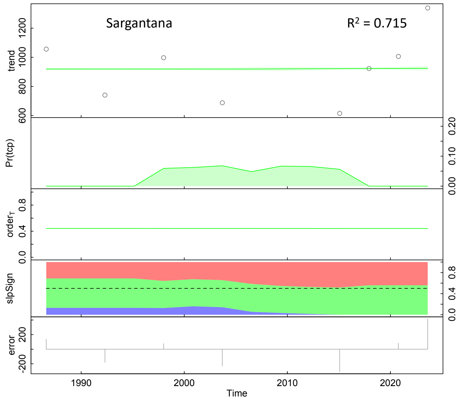
BEAST decomposition and changepoint detection
