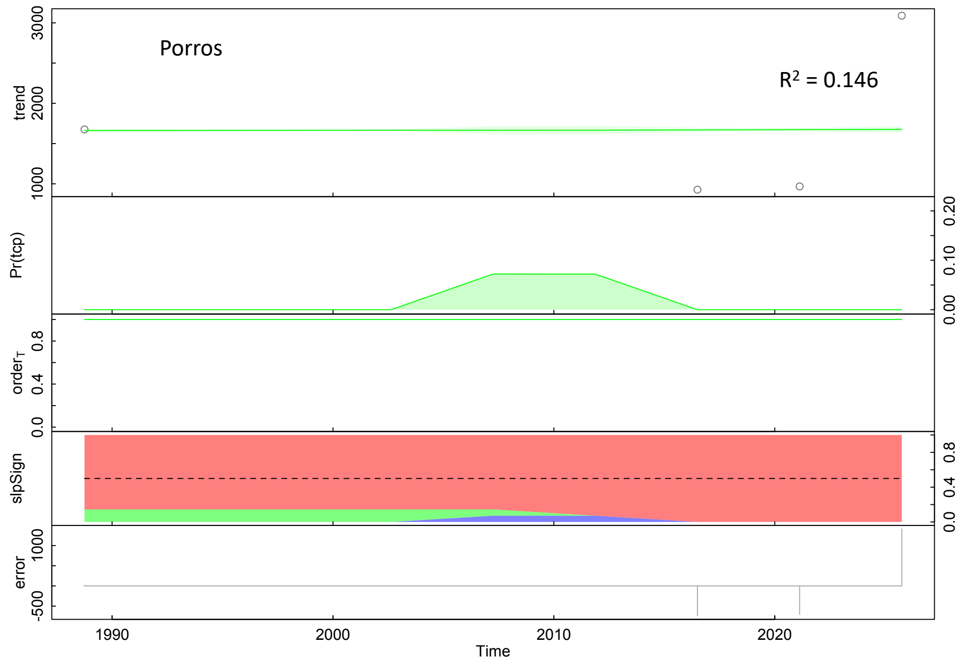
BEAST decomposition and changepoint detection
