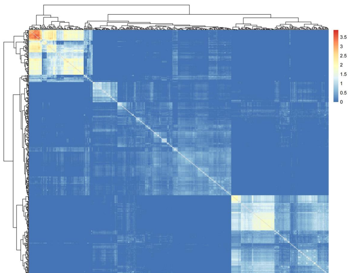
Supplementary Figure 1. 437 Tobacco germplasm kinship heat map.
