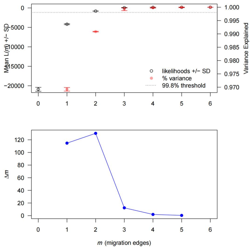
Supplementary Figure 2. Variance explained analysis of gene flow.
