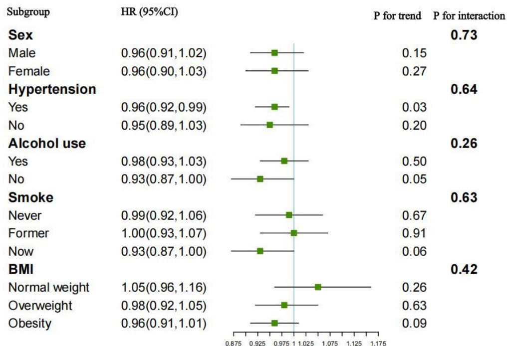
Subgroup analysis of the association between dietary OBS and all-cause mortality
