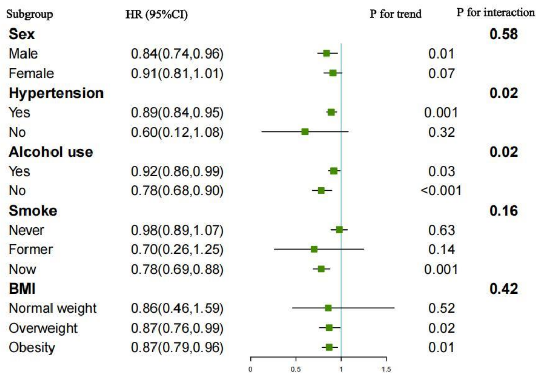
Subgroup analysis of the association between dietary OBS and CVD mortality
