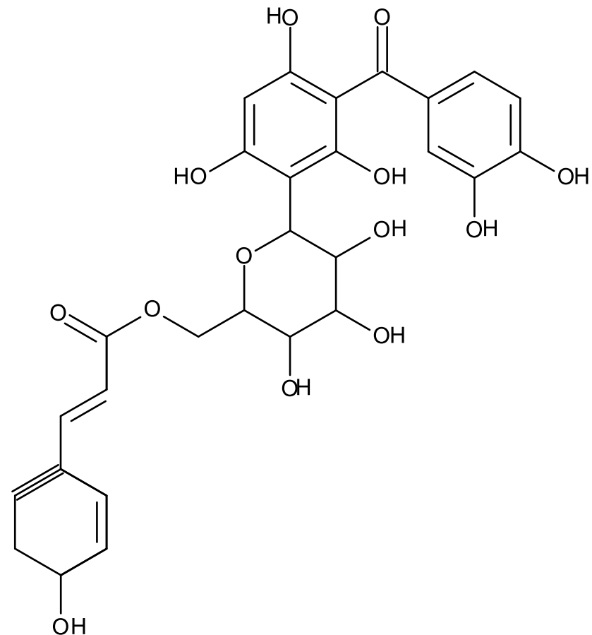
Maclurin-3-C-6''-O-p-coumaroyl glucoside (5)
