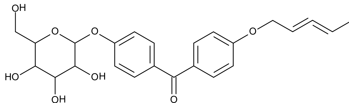
4'-pentadienyloxy benzophenone-3-O-glucoside (21)
