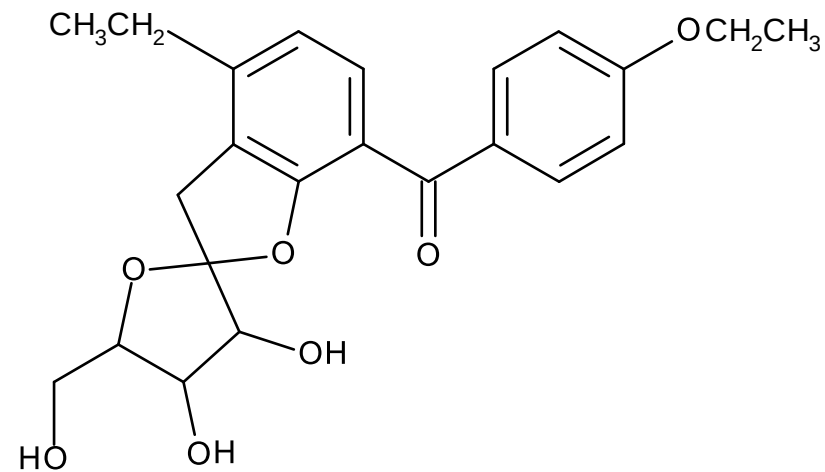
4-Ethyl-4'-ethoxybenzophenone-2-O-(2''),3-C-(1'')-1''-desoxy-fructofuranoside (31)
