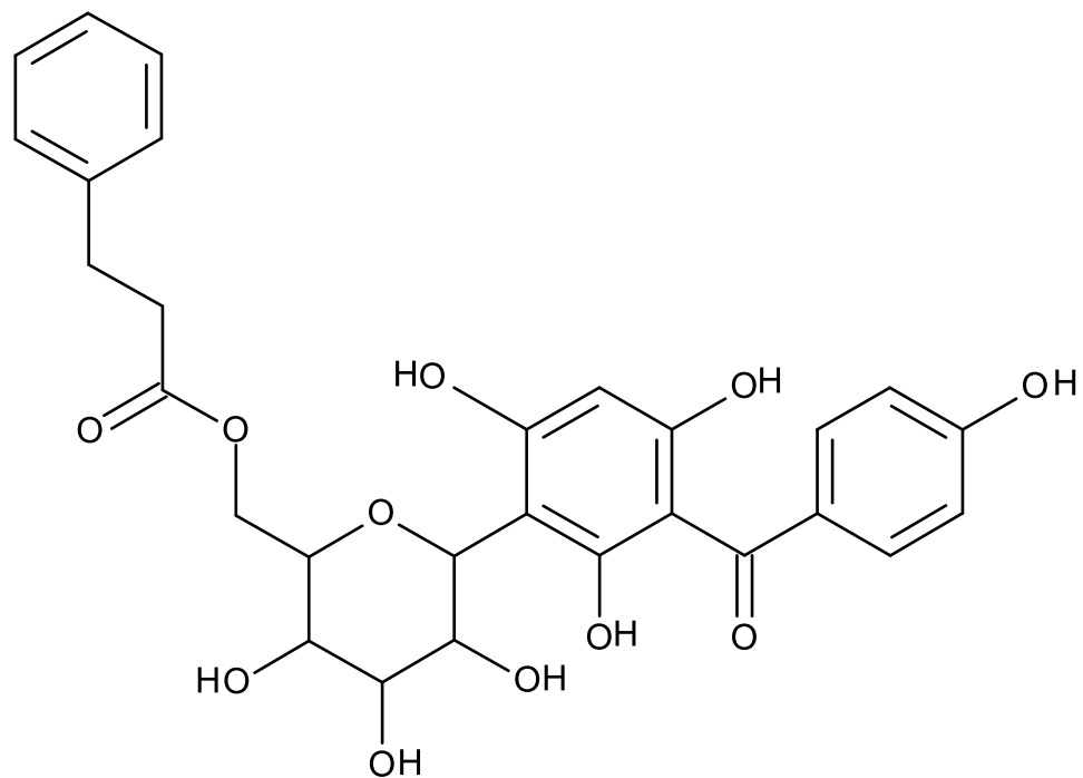
iriflophenone-3-C-6''-O-hydrocinnamyl glucoside (11)
