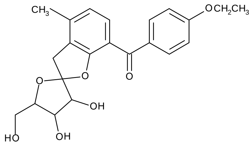
4-Methyl-4'-ethoxybenzophenone-2-O-(2''),3-C-(1'')-1''-desoxy-fructofuranoside (30)
