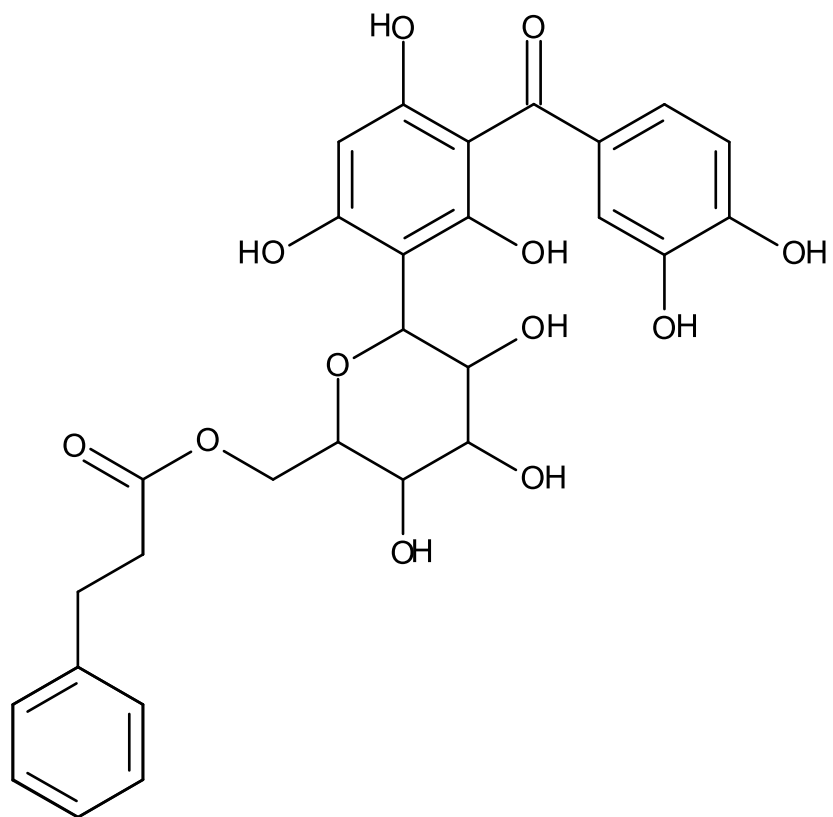
Maclurin-3-C-6''-O-hydrocinnamyl glucoside (1)
