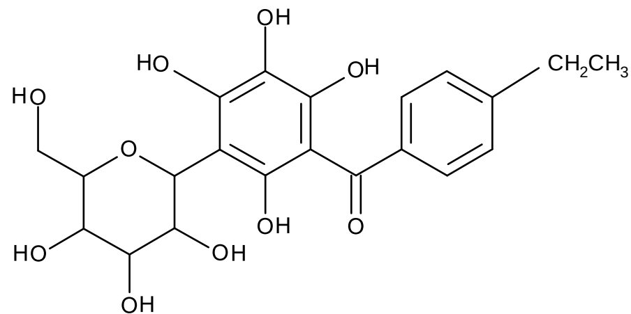
2,4,5,6-tetrahydroxy-4'-ethyl-benzophenone-3-C-glucoside (8)
