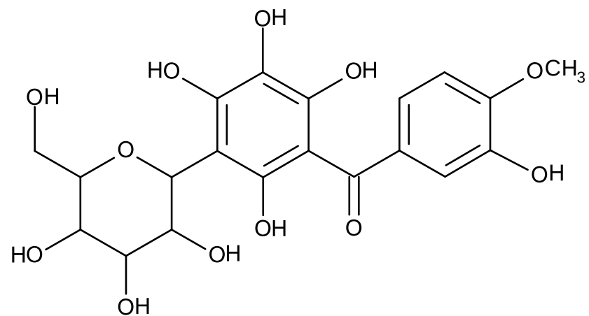
2, 3',4,5,6-pentahydroxy-4'-methoxy-benzophenone-3-C-glucoside (32)
