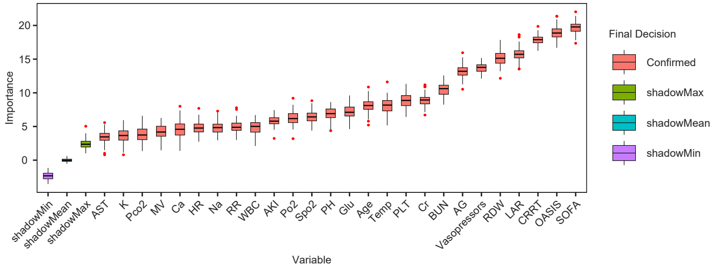
Boruta Feature Filtering Each Variable Importance Box Plot
