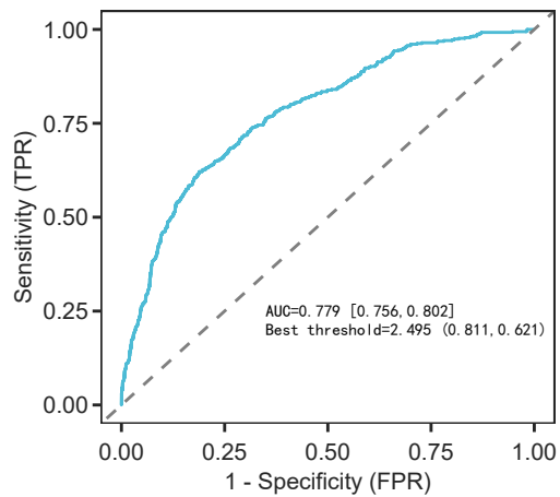
ROC Curve Plot
