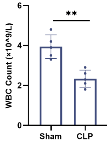
Figure s7 Validation of the establishment of CLP mouse model. White blood cell counts measured 12 hours after CLP surgery were significantly lower in CLP mice than in sham mice (n=5). Data is presented as mean \pm SD, and an unpaired Student's t-test was applied to determine the statistical significance among the groups. **P<0.01.
