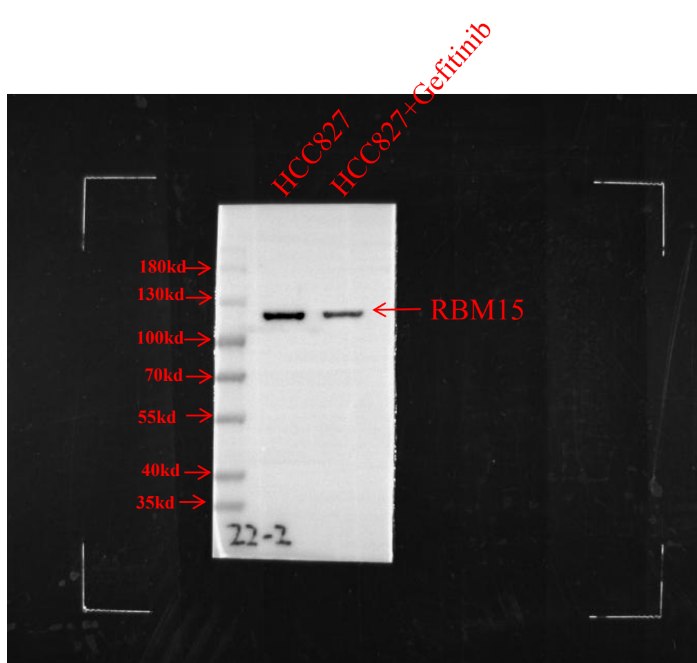
Fig3-B- RBM15
