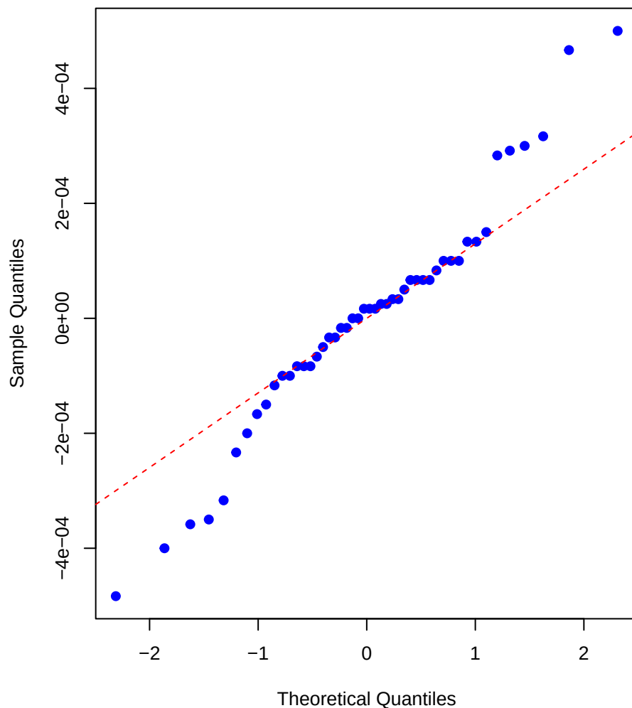
Silver (Ag) – Q-Q Plot
