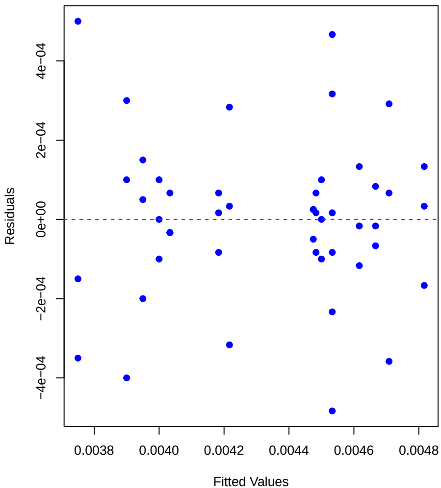
Silver (Ag) – Residuals vs Fitted
