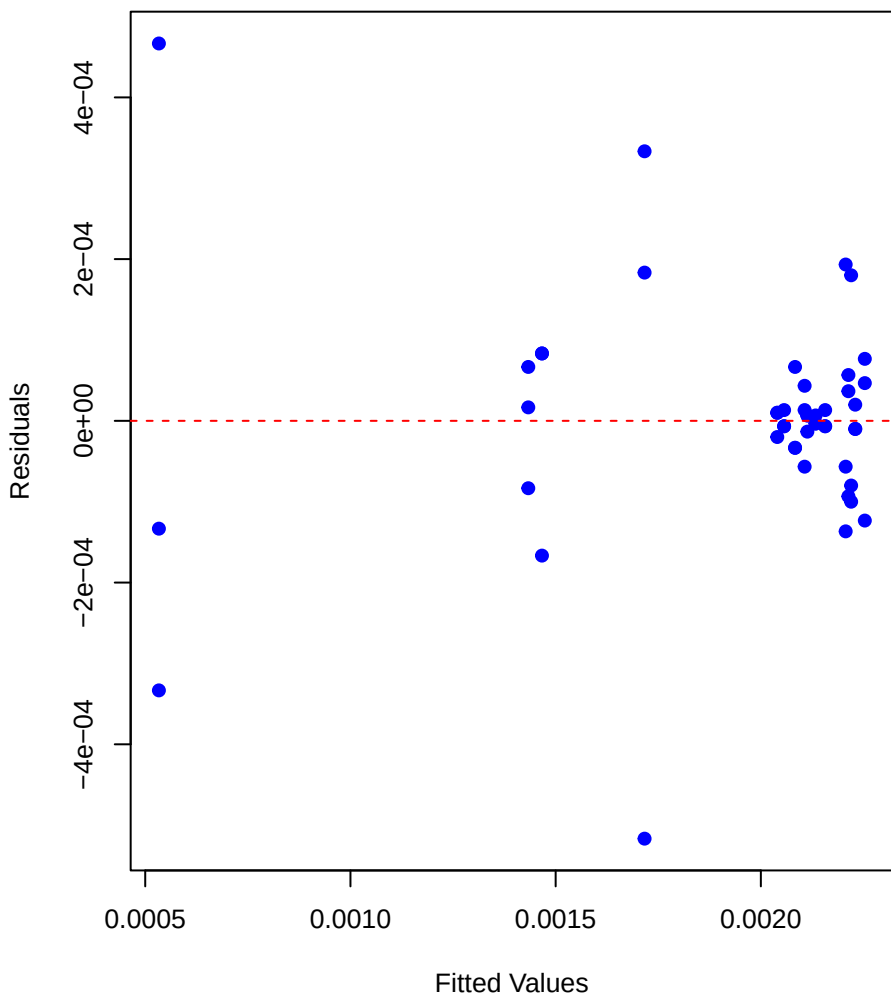
Zinc (Zn) – Residuals vs Fitted
