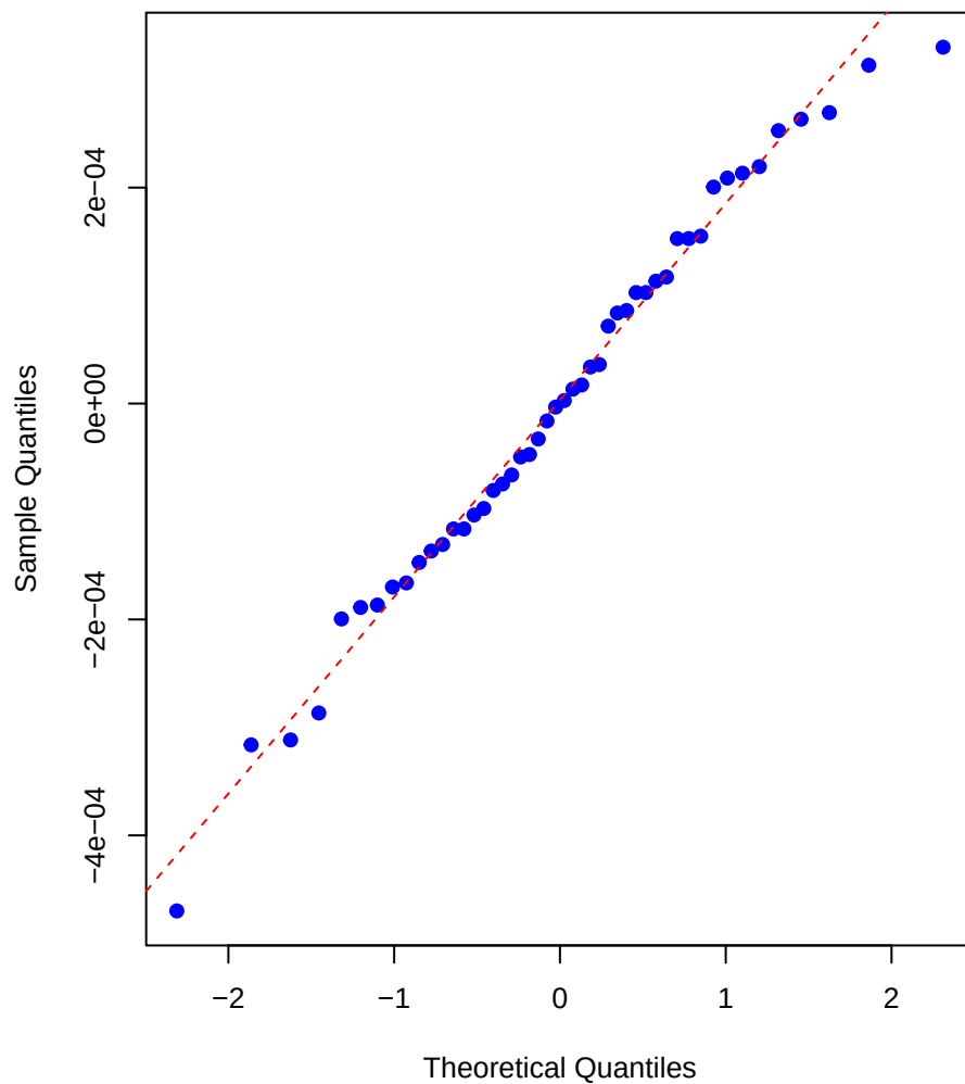
Copper (Cu) – Q-Q Plot
