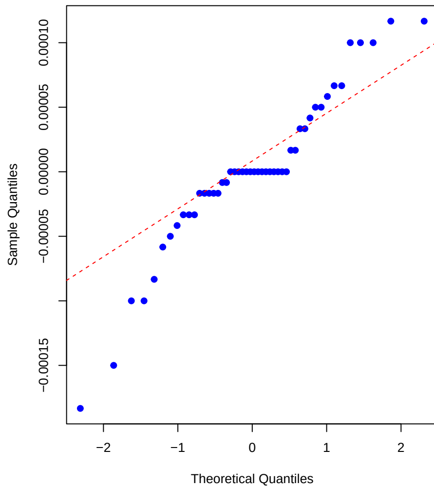
Iron (Fe) – Q-Q Plot
