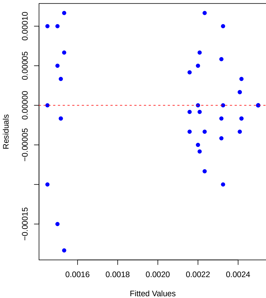
Iron (Fe) – Residuals vs Fitted
