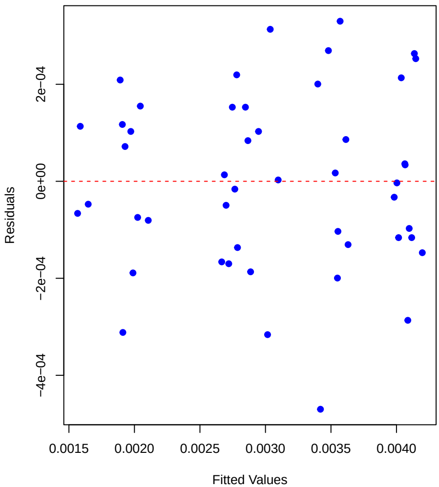
Copper (Cu) – Residuals vs Fitted
