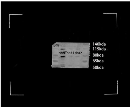
Fig5E-F13A1
