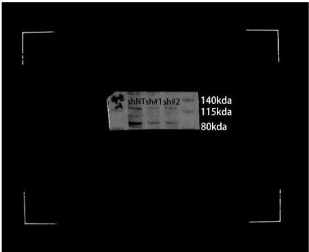
Fig5E-N-cadherin
