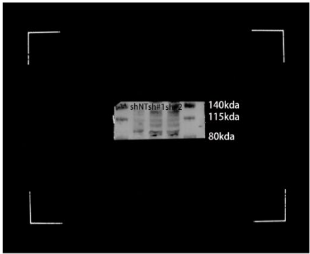
Fig5E-E-cadherin
