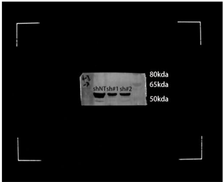
Fig5E-E-cadherin
