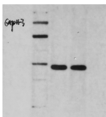
Supplementary FIG.1.A GAPDH
