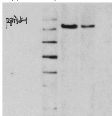
Supplementary FIG.2.D P-PI3K
