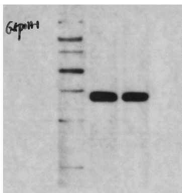
Supplementary FIG.2.D GAPDH
