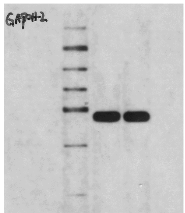
Supplementary FIG.1.E GAPDH
