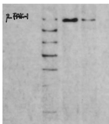
Supplementary FIG.2.D FAK
