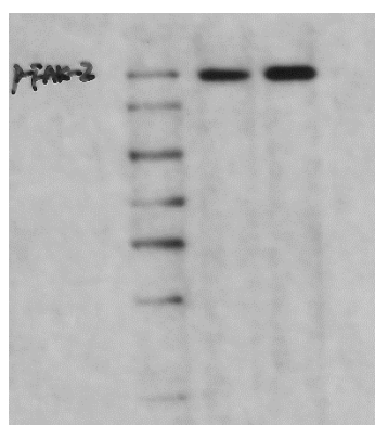
Supplementary FIG.1.E p-FAK
