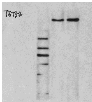
Supplementary FIG.1.E p-FAK
