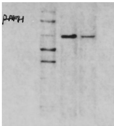
Supplementary FIG.2.D AKT
