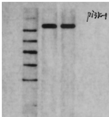
Supplementary FIG.2.D P-AKT
