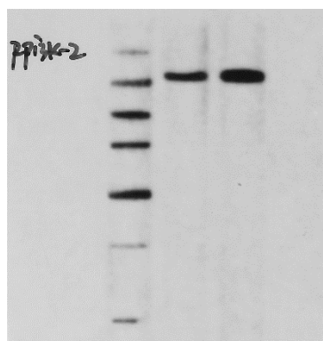
Supplementary FIG.1.E p-AKT
