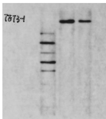
Supplementary FIG.2.D P-FAK
