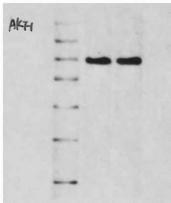
Supplementary FIG.2.D GAPDH
