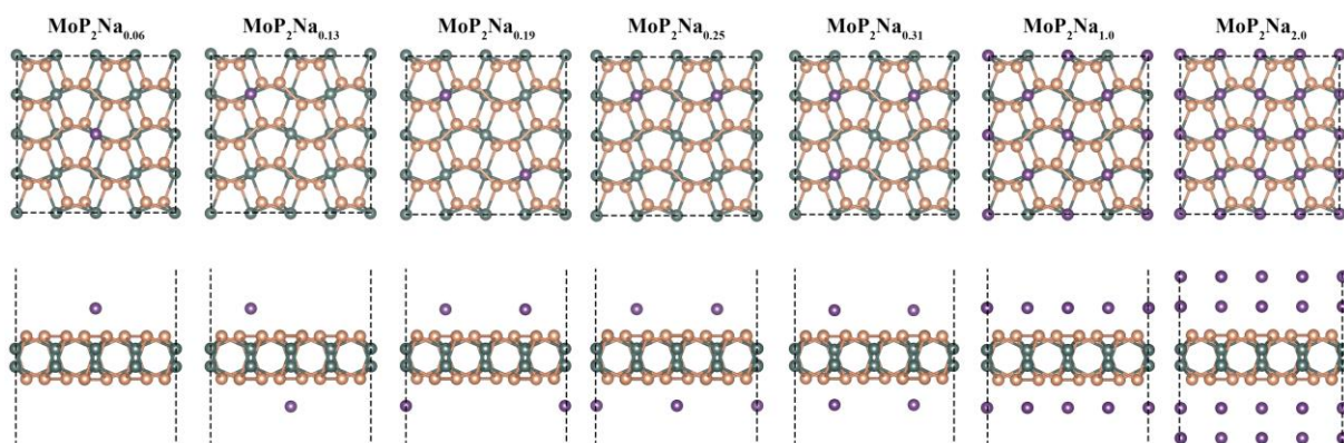
Supplementary Figure 1. The thermodynamically stable MoP 2 Na m structures.
