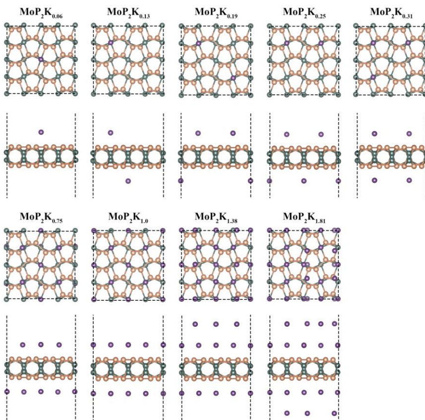
Supplementary Figure 2. The thermodynamically stable MoP 2 K m structures.
