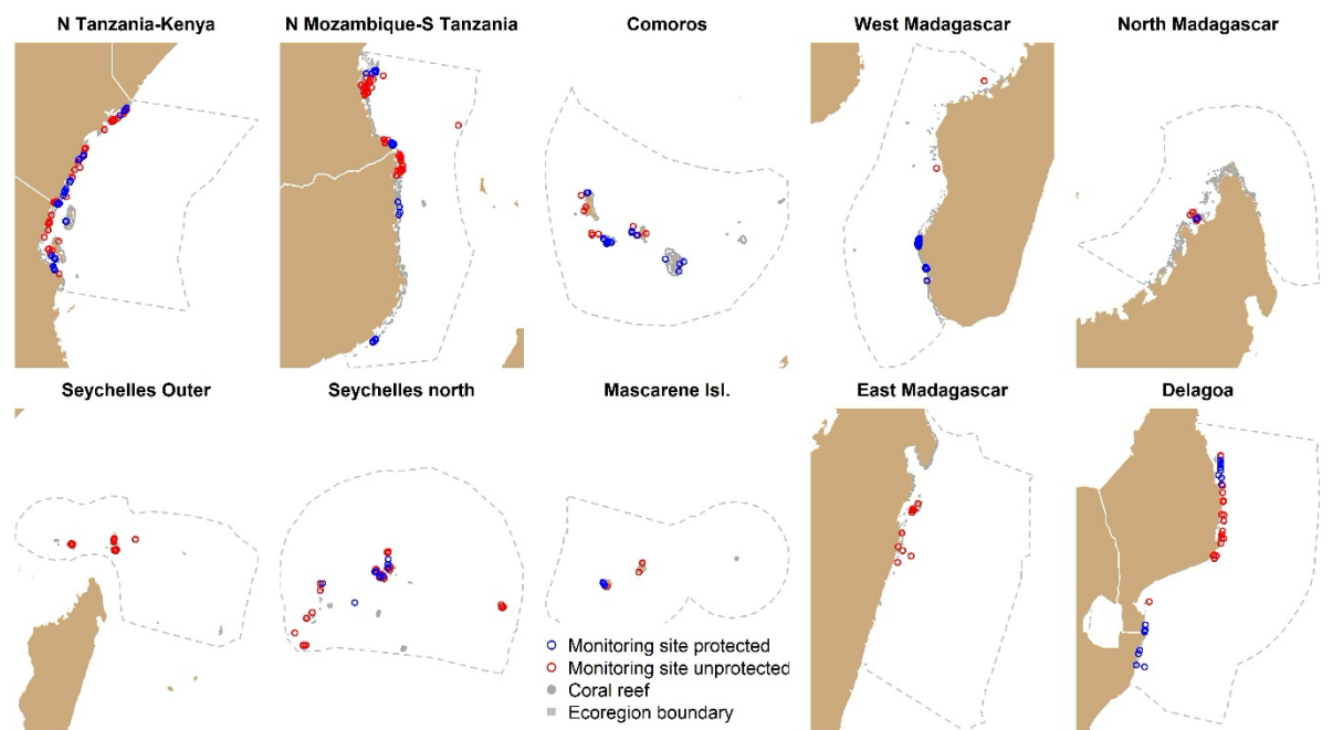
Figure S3. Distribution of benthic monitoring sites across coral reefs (grey) in the 10 eco-regions with data. Blue circles are sites within protected areas and red circles are unprotected sites. Algae and fish data were obtained from smaller subsets of these sites.
