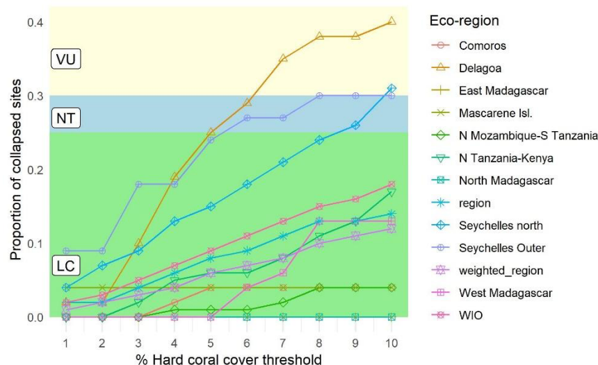
Figure S2. Sensitivity analysis of Criterion A assessment to the collapse threshold for coral cover varying from 1% to 10%.
