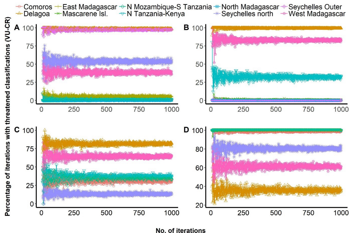
Figure S4. Repeated sampling trials to determine number of iterations to produce stable percentage of threatened classifications (VU-CR), from 10 to 1000 (x axis) for each of the following indicators. A: hard coral cover; B: algae:coral ratio; C: parrotfish; D: grouper.
