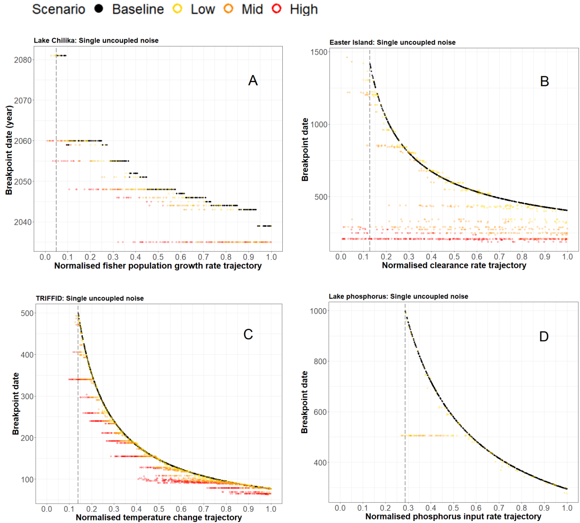
Figure S4-11: Scatter plots depicting the raw data producing the boxplots in Figure S4-5. The dashed grey vertical line represents the weakest primary driver value associated with an ATDC in each plot. Subplots: (A) Lake Chilika model outputs, primary slow driver: fisher population growth; (B) Easter Island model outputs, primary slow driver = tree clearance; (C) TRIFFID model outputs, primary slow driver = temperature change; (D) Lake phosphorus model outputs, primary slow driver = phosphorus input. Model timestep units are the same as in Figure S2-1.
