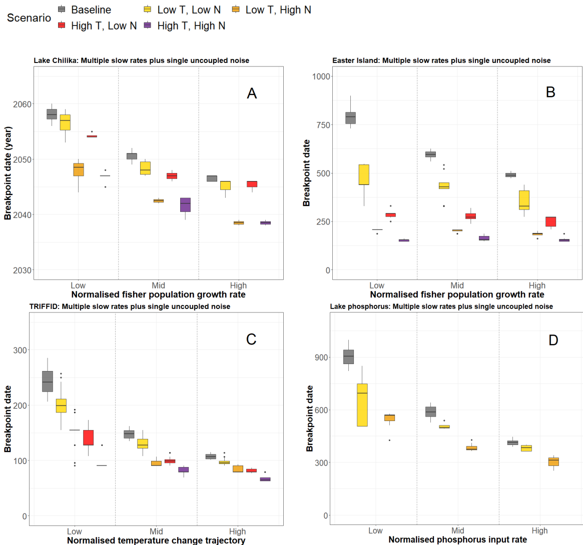
Figure S4-6: The relationship between the breakpoint date and the primary slow driver (grey) when weak (normalised T values \leq 0.333 ) and strong (normalised T values > 0.666 ) multiple driver trajectories are combined with weak (normalised \sigma values \leq 0.333 ) and strong (normalised \sigma values > 0.666 ) uncoupled noise (T = trajectory, N = noise). The breakpoint date is defined by the second alternative method described above (Type 2a boundaries). As in the main manuscript (i.e., Figures 2-4), the normalised primary driver trajectories are apportioned into three discrete ranges: ‘low’ – 0.25-0.35, ‘mid’ – 0.45-0.55, and ‘high’ – 0.65-0.75. For comparison with the main manuscript, this figure is the equivalent of Figure 4. Subplots: (A) the Lake Chilika model, primary slow driver = fisher population growth, additional driver: climate change and fish price; (B) the Easter Island model, primary slow driver = tree clearance, additional drivers: agricultural carrying capacity and tree mortality; (C) the TRIFFID model, primary slow driver = temperature change, additional driver: disturbance rate; (D) the Lake phosphorus model, primary slow driver = phosphorus, additional drivers: phosphorus recycling rate, phosphorus sedimentation rate. Note, the first 10,000 simulations of the Lake phosphorus model (subplot D) did not produce any outcomes between the 0.25-0.35, 0.45-0.55 and 0.65-0.75 primary driver ranges within the ‘high trajectory, high noise’ scenario. Model timestep units are the same as in Figure S2-1. Boxplots dimensions are as Figure 2. The number of simulations (n) underpinning each primary driver trajectory range (i.e., low, middle, and high) in each of the above subplots are as follows: (A) 45, 60 and 43; (B) 82, 96 and 94; (C) 340, 330 and 315; (D) 75, 95 and 65.
