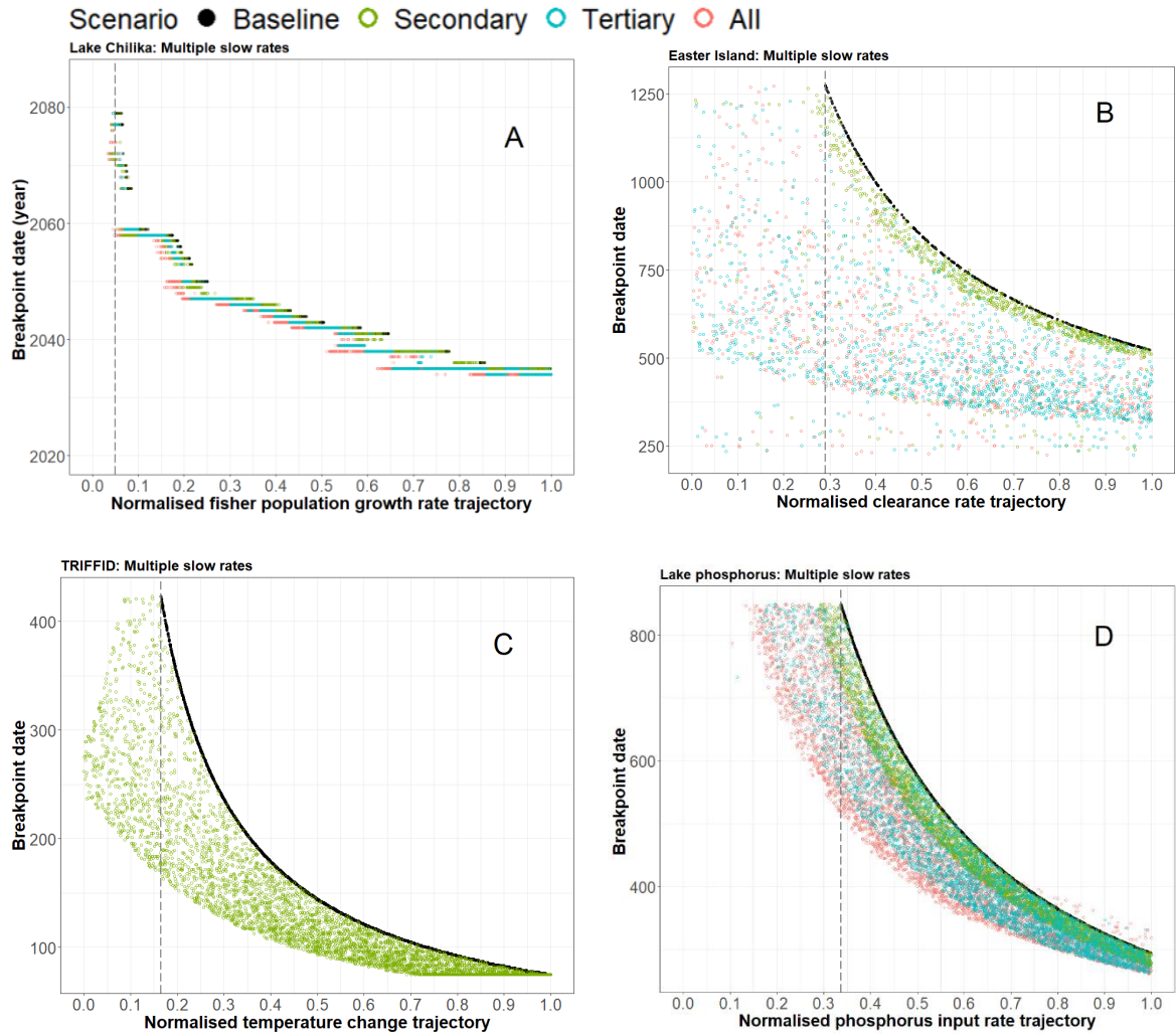
Figure S2-4: Scatter plots depicting the raw data producing the boxplots in Figure 2 of the main manuscript. The dashed grey vertical line represents the weakest primary driver value associated with an ATDC in each plot. Subplots: (A) Lake Chilika model outputs, primary slow driver: fisher population growth; (B) Easter Island model outputs, primary slow driver = tree clearance; (C) TRIFFID model outputs, primary slow driver = temperature change; (D) Lake phosphorus model outputs, primary slow driver = phosphorus input. Model timestep units are the same as in Figure S2-1.
