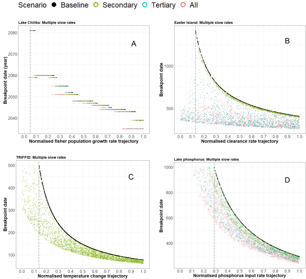
Figure S4-10: Scatter plots depicting the raw data producing the boxplots in Figure S4-4. The dashed grey vertical line represents the weakest primary driver value associated with an ATDC in each plot. Subplots: (A) Lake Chilika model outputs, primary slow driver: fisher population growth; (B) Easter Island model outputs, primary slow driver = tree clearance; (C) TRIFFID model outputs, primary slow driver = temperature change; (D) Lake phosphorus model outputs, primary slow driver = phosphorus input. Model timestep units are the same as in Figure S2-1.
