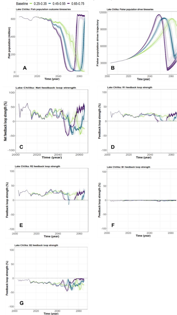
Figure S6-1: Timeseries outcomes from the first LTM experiment (Lake Chilika model), where the baseline driver strength was increased over three trajectory ranges. See Table S6-1 for descriptions of the two reinforcing (subplots D-E) and two balancing feedbacks (subplots F-G) responsible for driving the dynamics of the fish population (subplot A) over time. Subplots: (A) Timeseries of the modelled Lake Chilika fish population; (B) Timeseries of the primary driver (fisher population); (C) Timeseries of the net feedback loop strength (i.e., reinforcing minus balancing strengths); (D) Timeseries of percentage contribution of feedback R1 to model behaviour; (E) Timeseries of percentage contribution of feedback R2 to model behaviour; (F) Timeseries of percentage contribution of feedback B1 to model behaviour; (G) Timeseries of percentage contribution of feedback B2 to model behaviour. Simulations that are within \pm 0.5\% of the median primary driver trajectory are given a transparency value of 1 (i.e., opaque), while all other simulations are given a transparency (alpha value) of 0.05 in the R package 'ggplot'.
