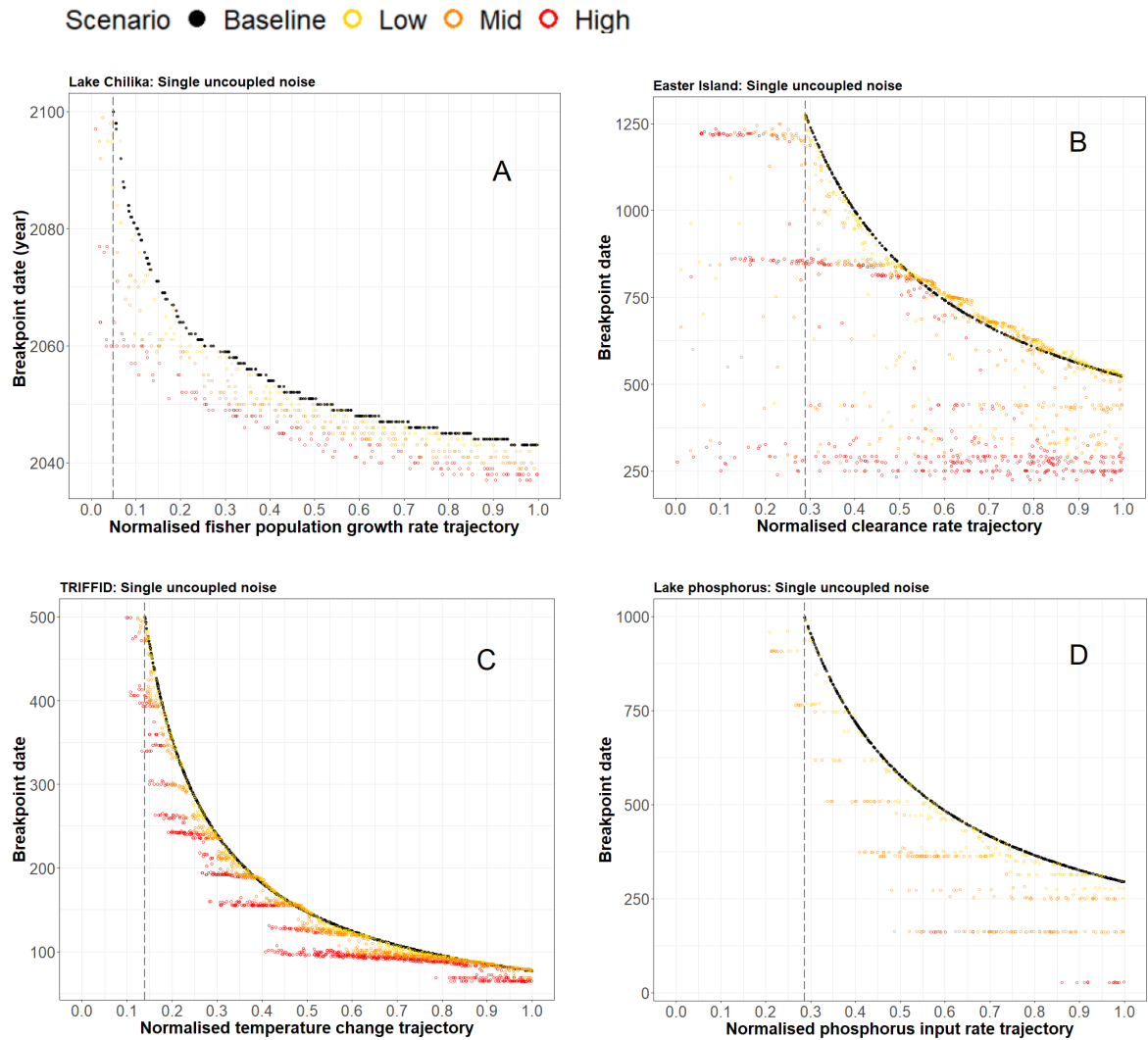
Figure S4-8: Scatter plots depicting the raw data producing the boxplots in Figure S4-2. The dashed grey vertical line represents the weakest primary driver value associated with an ATDC in each plot. Subplots: (A) Lake Chilika model outputs, primary slow driver: fisher population growth; (B) Easter Island model outputs, primary slow driver = tree clearance; (C) TRIFFID model outputs, primary slow driver = temperature change; (D) Lake phosphorus model outputs, primary slow driver = phosphorus input. Model timestep units are the same as in Figure S2-1.
