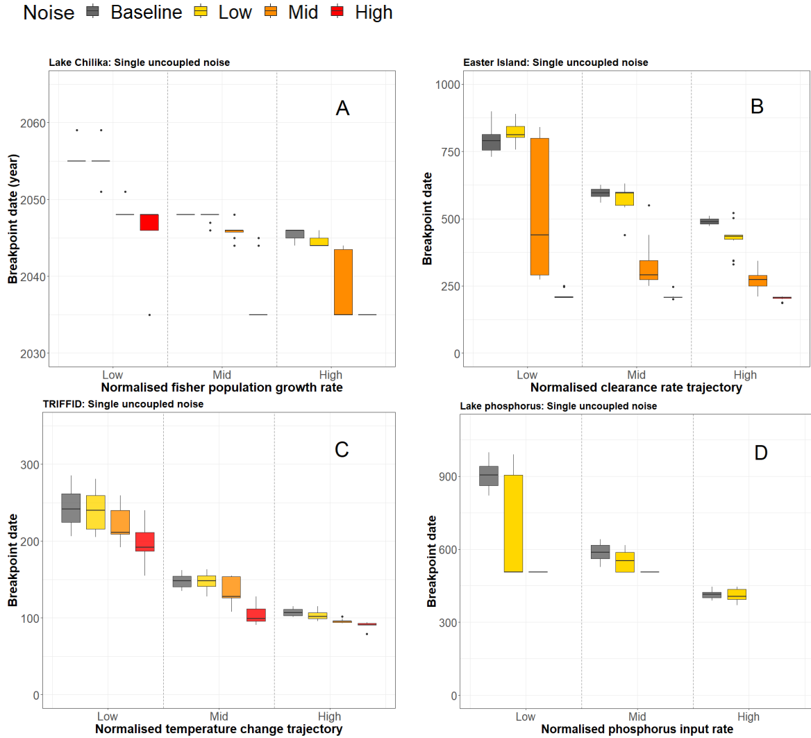
Figure S4-5: The relationship between the breakpoint date and the primary slow driver (grey) for varying levels of uncoupled noise in the primary slow driver ( \sigma ), where normalised \sigma values \leq 0.333 signify ‘low noise’ (yellow), normalised \sigma values > 0.333 and \leq 0.666 signify ‘mid noise’ (orange), and normalised \sigma values > 0.666 signify ‘high noise’ (red) (Methods Section 2.3). The breakpoint date is defined by the second alternative method described above (Type 2a boundaries). As in the main manuscript (i.e., Figures 2-4), the normalised primary driver trajectories are apportioned into three discrete ranges: ‘low’ – 0.25-0.35, ‘mid’ – 0.45-0.55, and ‘high’ – 0.65-0.75. For comparison with the main manuscript, this figure is the equivalent of Figure 3. Subplots: (A) Lake Chilika model outputs, primary slow driver = fisher population growth; (B) Easter Island model outputs, primary slow driver = tree clearance; (C) TRIFFID model outputs, primary slow driver = temperature change; (D) Lake phosphorus model outputs, primary slow driver = phosphorus input. Model timestep units are the same as in Figure S2-1. Boxplot dimensions are as Figure 2. The number of simulations ( n ) underpinning each primary driver trajectory range (i.e., low, middle, and high) in each of the above subplots are as follows: (A) 78, 82 and 79; (B) 88, 120 and 140; (C) 409, 401 and 389; (D) 86, 135 and 140.
