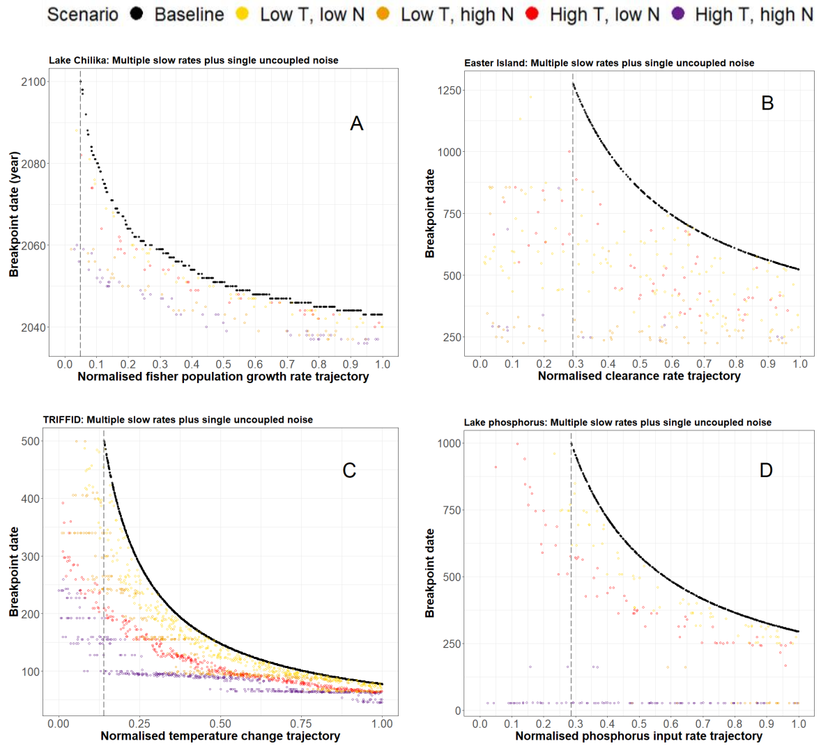
Figure S4-9: Scatter plots depicting the raw data producing the boxplots in Figure S4-3. The dashed grey vertical line represents the weakest primary driver value associated with an ATDC in each plot. Subplots: (A) Lake Chilika model outputs, primary slow driver: fisher population growth; (B) Easter Island model outputs, primary slow driver = tree clearance; (C) TRIFFID model outputs, primary slow driver = temperature change; (D) Lake phosphorus model outputs, primary slow driver = phosphorus input. Model timestep units are the same as in Figure S2-1.
