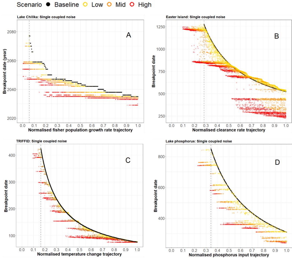
Figure S2-8: Scatter plots depicting the raw data producing the boxplots in Figure S2-2. The dashed grey vertical line represents the weakest primary driver value associated with an ATDC in each plot. Subplots: (A) Lake Chilika model outputs, primary slow driver: fisher population growth; (B) Easter Island model outputs, primary slow driver = tree clearance; (C) TRIFFID model outputs, primary slow driver = temperature change; (D) Lake phosphorus model outputs, primary slow driver = phosphorus input. Model timestep units are the same as in Figure S2-1.
