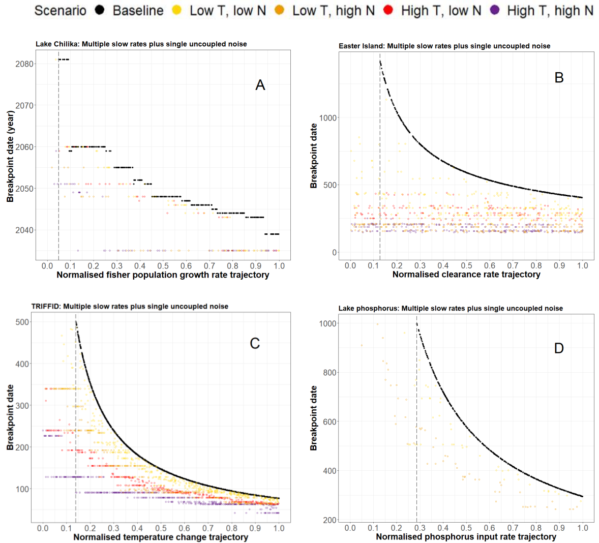
Figure S4-12: Scatter plots depicting the raw data producing the boxplots in Figure S4-6. The dashed grey vertical line represents the weakest primary driver value associated with an ATDC in each plot. Subplots: (A) Lake Chilika model outputs, primary slow driver: fisher population growth; (B) Easter Island model outputs, primary slow driver = tree clearance; (C) TRIFFID model outputs, primary slow driver = temperature change; (D) Lake phosphorus model outputs, primary slow driver = phosphorus input. Model timestep units are the same as in Figure S2-1.
