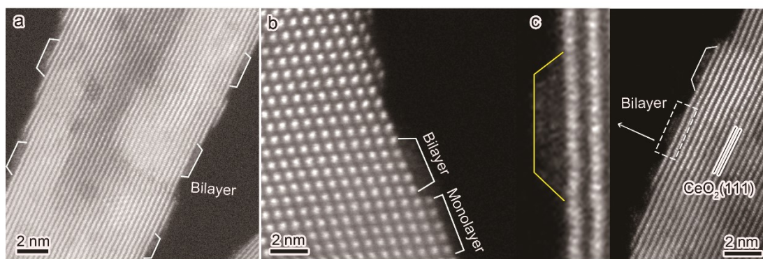
Supplementary Figure 6. Atom-resolved HAADF-STEM images of the Cu-773 catalyst. Copper monolayers, bilayers and trilayers were clearly seen; the inset in c is an enlarged image that shows the atomic arrangement in a typical copper bilayer that is dominantly presented in the sample.
