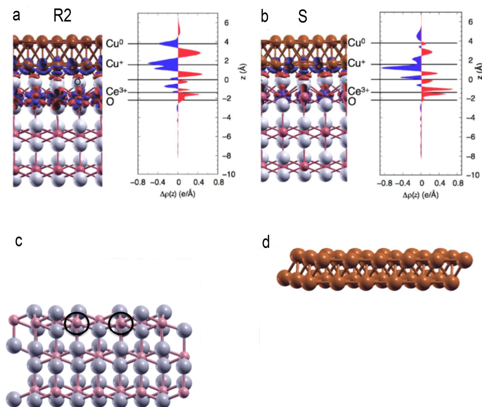
Supplementary Figure 11. Fully-relaxed structures of the R2 (a) and S (b) systems and calculated bonding charge \Delta p(r) that corresponds to the plane-integrated bonding charge \Delta p(z) across the interfaces. The red and blue areas represent charge accumulation and depletion, respectively. Color
