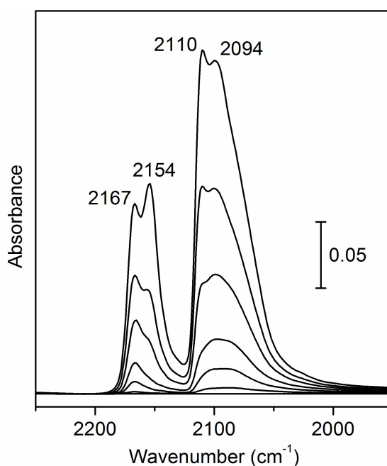
Supplementary Figure 9. IR spectra recorded upon exposing the Cu-473 catalyst to CO at 80 K and gradually increasing the pressure of CO from 1 \times 10^{-5} to 1 \times 10^{-2} mbar.
