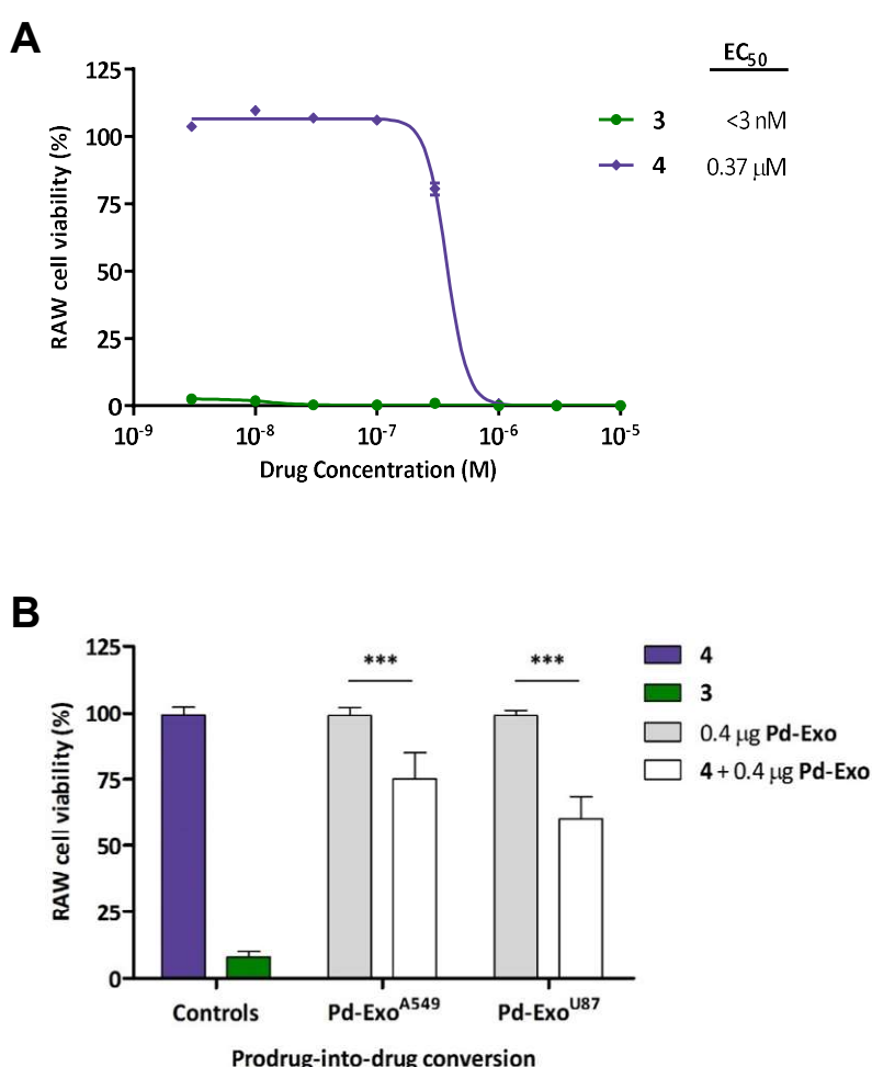
Suppl. Fig. 20. (A) RAW 264.7 dose-response curves after 5 d treatment with 3 and 4 . Curves fit: sigmoidal variable slope curves. Error bars: \pm SEM, n = 3 . (B) Pd-Exo -mediated uncaging of 4 inside RAW 264.7 cells. Cells were incubated for 6 h with 0.4 \mu g / 100 \mu L of either Pd-Exo A549 or Pd-Exo U87 . Cells were thoroughly washed to eliminate extracellular vesicles followed by addition of prodrug 4 (0.2 \mu M). Controls: Pd-Exo A549 / Pd-Exo U87 only (–ve control, grey); prodrug 4 only (–ve control, purple); 3 (+ve control, green). Cell viability was measured at day 5 using PrestoBlue. Error bars: \pm SEM, n = 3 . *** P < 0.001 (ANOVA).
