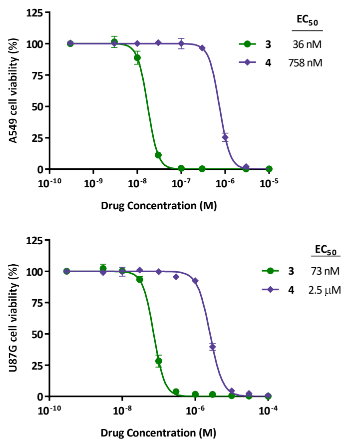
Suppl. Fig. 15. Dose-response curves after 5 d treatment with 3 and 4 in A549 (top) and U87 cells (bottom). Curves fit: sigmoidal variable slope curves. Error bars: ± SEM, n = 3.
