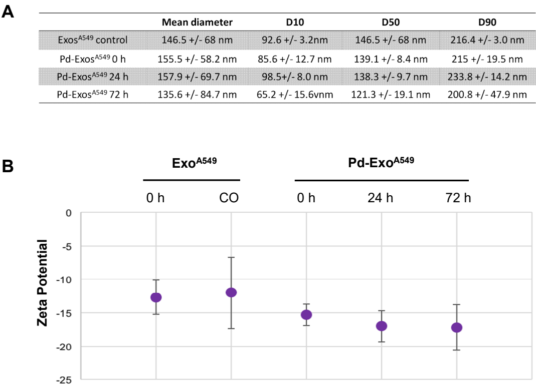
Suppl. Fig. 7. Stability study. (A) Particle size analysis of Exo A549 ( t= 0h ) and Pd-Exo A549 ( t= 0, 24 and 72 h ). Error bars: \pm SD , n = 3 . (B) Zeta potential analysis of Exo A549 (before and after treatment with CO) and Pd-Exo A549 ( t= 0, 24 and 72 h ). Error bars: \pm SD , n = 2 .
