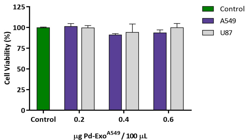
Suppl. Fig. 11. A549 and U87 cell viability study after treatment with Pd-Exo A549 . Cell viability was measured at day 5 using PrestoBlue® reagent. Error bars: ± SEM, n = 3.
