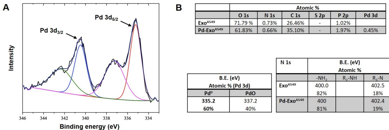
Suppl. Fig 5. (A) X-Ray Photoelectron Spectroscopy (XPS) spectrum of Pd-Exo A549 . (B) XPS analysis of Exo A549 and Pd-Exo A549 . The top table indicates the atomic composition percentage of Exo A549 and Pd-Exo A549 . The bottom left and right tables show the oxidation state of Pd 3d atoms of Pd-Exo A549 and N 1s atoms of Exo A549 and Pd-Exo A549 , respectively.
