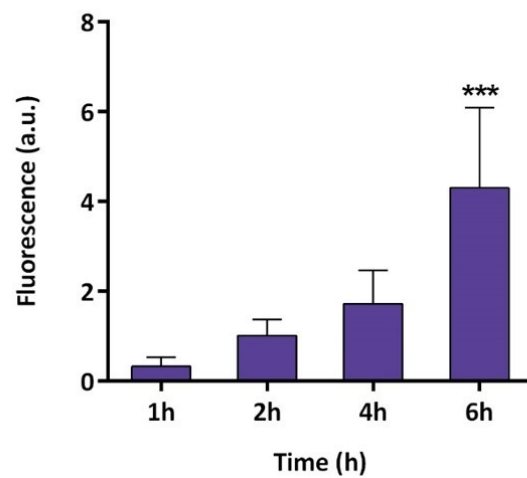
Suppl. Fig. 13. Merged confocal images of A549 cells after treatment with Pd-Exo A549 for 1 h, 2 h, 4 h and 6 h. Actin fibers (phalloidin-488) are shown in green, cell nuclei (Draq5) in blue and clusters of Pd-Exo A549 in red. Scale bar= 50 \mu m. Lower panel: Quantitative analysis of red fluorescent intensity in the cells at different timepoints. Error bars: \pm SD, n = 2 .
