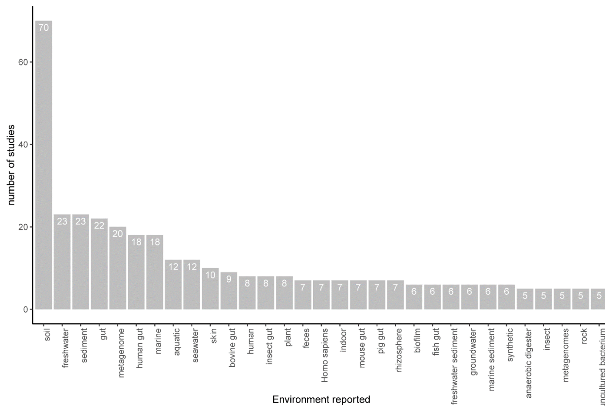
Supplementary Figure 4. Environments targeted by studies sequencing the V3-V4 region of the 16S rRNA gene. We selected the 441 V3-V4 studies for which sequence data and metadata was available. Environment metadata was extracted from the ‘ScientificName’ attribute of the metadata files obtained from NCBI. Only environments which were listed in at least 5 studies are included. Among the 441 studies, 172 distinct environments were reported. Note that 25 studies listed the environment as ‘metagenome(s)’, and different degrees of ambiguity exist in listing the environment (i.e., gut and Homo sapiens vs. human gut).
