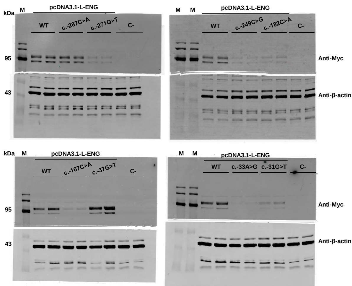
Supplementary Figure 2. Western blot results on total proteins extracted from transfected HeLa cells with 1 µg of pcDNA3.1-L-ENG constructs containing ENG variants at the origin of uAUGs in frame with the same stop codon at position c.125. The blots correspond to the uncropped upper and lower blots in main Figure 2b. Each blot was cut in 2 parts and each part was incubated with the corresponding antibody: monoclonal anti-(c-Myc Tag) or anti-β-actin as a loading control. Specific fluorescent secondary antibodies were used. Finally, Odyssey Infrared Imaging System (Li-Cor Biosciences) in 700 and 750 channels was used to scan, reveal, and quantify the blots. HeLa cell extracts were analyzed in duplicates. kDa, kilodalton; M, protein ladder; WT, wild-type, C-, negative control corresponding to pcDNA3.1- empty vector.
