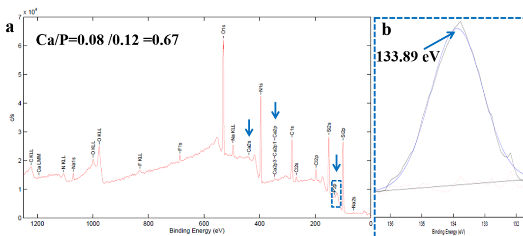
Supplementary Figure 1. The in situ synthesized particles are characterized by post-situ XPS. The deconvoluted P high energy resolution peak matches with the photoelectron line of 2p 3/2 of P in CaP.
