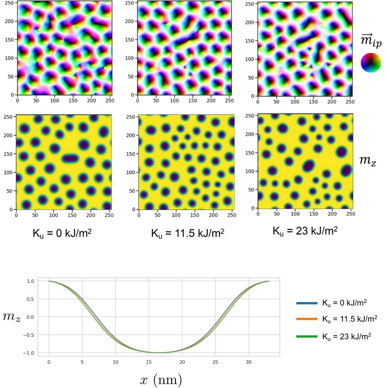
Figure S16: Results of micromagnetic simulations for skyrmion with the experimentally measured M_s = 253 \text{ kA m}^{-1} , A_{ex} = 0.69 \text{ pJ m}^{-1} , for a 108 nm thick film in an external field of H = 0.16 \text{ T} . We chose a DMI D = 0.25 \text{ mJ m}^{-2} in order to get a skyrmion radius that matches our LTEM and MFM experiments. We show that the results are substantially independent of the magnetic anisotropy K_u . Our FMR measurements lead to K_u estimates in the range 11.5 - 23 kJ m -3 . The upper panels show the in-plane magnetization, the middle panels show m_z , while the lower panel shows line cuts of the spatial variation of m_z , from which we define the skyrmion diameter using the zero crossings.
