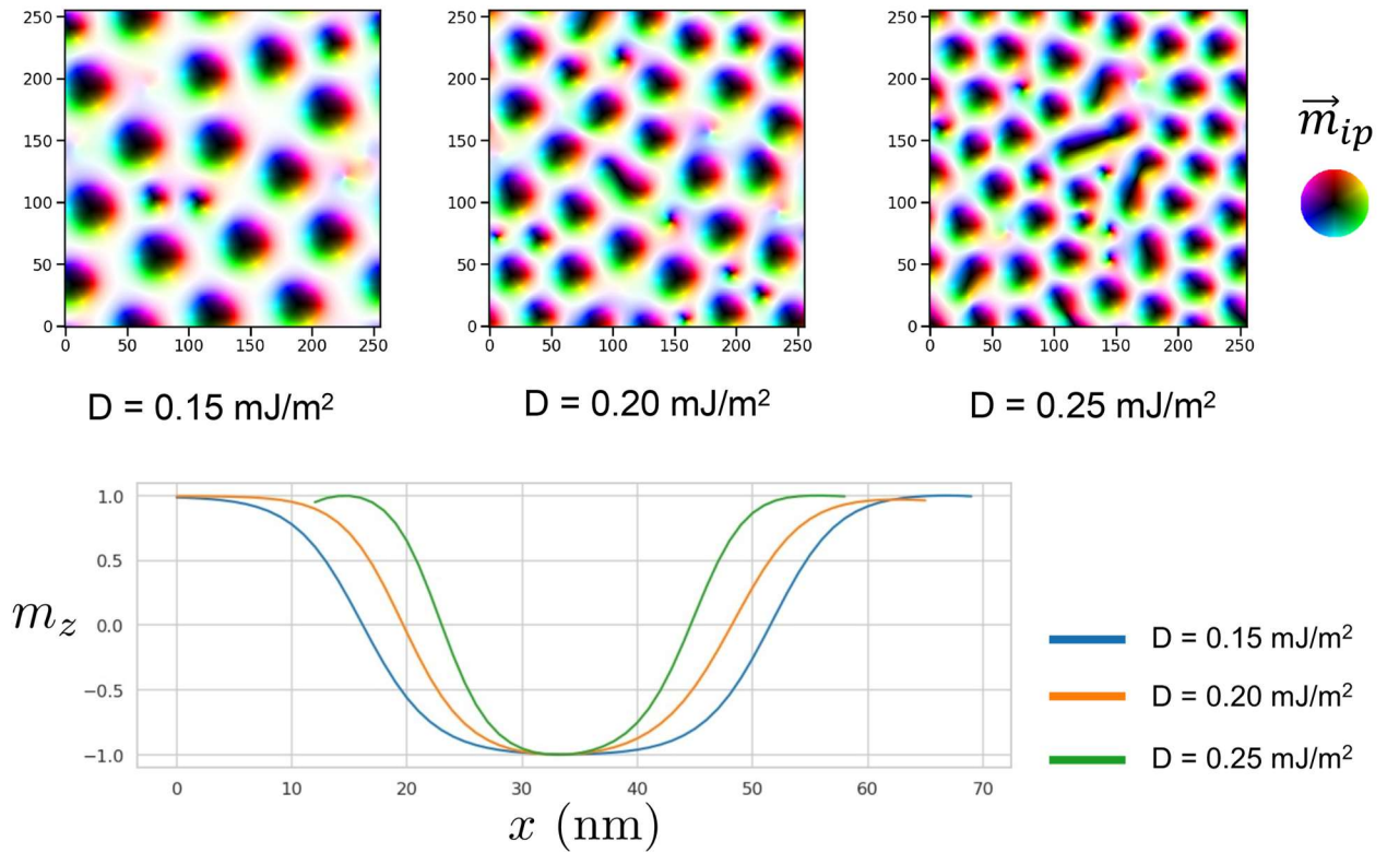
Figure S15: Results of micromagnetic simulations for skyrmion with the experimentally measured M_s = 253 kA m -1 , A_{ex} = 0.69 pJ m -1 , and K_u = 17 kJ m -3 for a 108 nm thick film in an external field of H = 0.16 T. We show results for three different DMI values. Choosing D = 0.25 mJ m -2 leads to skyrmions of 22 nm diameter, consistent with our LTEM and MFM experiments. The upper panels show the in-plane (ip) magnetization, and the lower panel shows line cuts of the spatial variation of m_z , from which we define the skyrmion diameter using the zero crossings.
