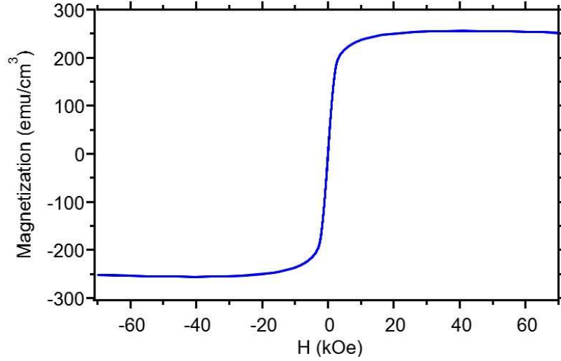
Figure S14. Out-of-plane hysteresis loop of 108 nm thick \text{Fe}_{1.2}\text{Ge} film, with diamagnetic background subtracted, obtained at 300 K via SQUID magnetometry.
