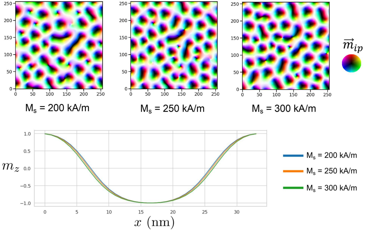
Figure S17: Results of micromagnetic simulations for skyrmion with the experimentally measured A_{ex} = 0.69 pJ m -1 , for a 108 nm thick film in an external field of H = 0.16 T. We chose a DMI D = 0.25 mJ m -2 and K_u = 17 kJ m -3 . The upper panels show the in-plane magnetization, while the lower panel shows the spatial variation of m_z , from which we define the skyrmion diameter using the zero crossings. The results for skyrmion size are substantially independent over a range of M_s values around the experimentally measured M_s = 253 kA m -1 .
