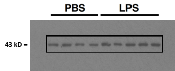
Extended Data Fig.7c: CD38
