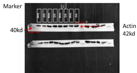
Fig 2a_β-actin_sample picture
