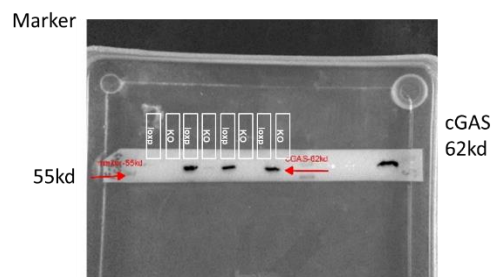
Fig 2a_cGAS_sample picture
