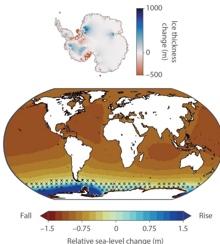
Figure S1. Pattern of global sea-level change due to a scenario of Antarctic ice volume gain.
