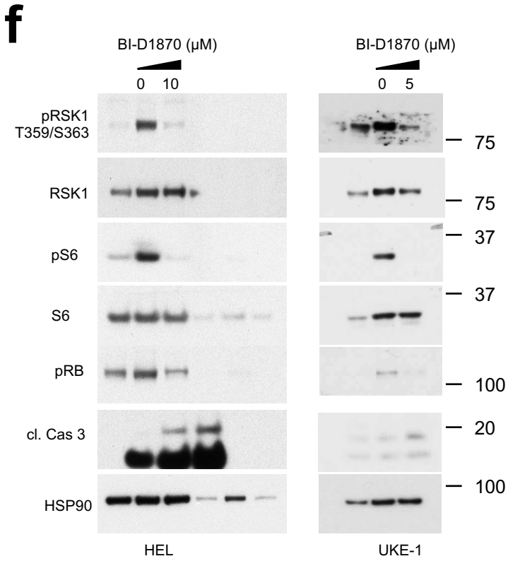
Fig. 4f. Immunoblot of HEL and UKE-1 cells treated with BI-D1870 or control for 24 hours.
