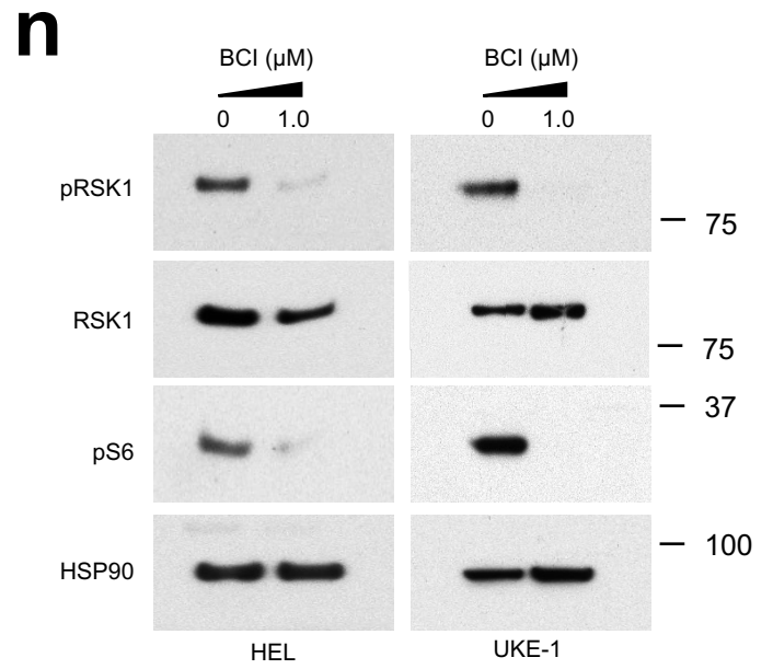
Fig. 4n. Immunoblot of HEL and UKE-1 cells treated with 1 \mu\text{M} BCI or control for 24 hours.
