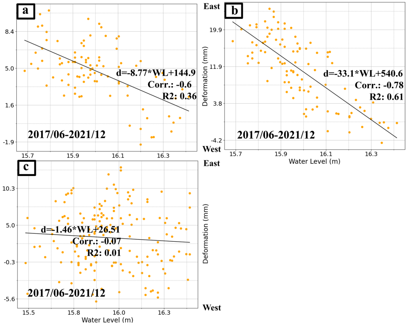
Supplementary Figure 2: Scatter plots depicting horizontal deformation relative to water level for points located on the bridge between polygons. (a) Scatter plot covering the period from June 2017 to December 2021 for points between polygons 1 and 2. (b) and (c) represent scatter plots for the same time frame, showing points between polygons 3 and 4, and between polygon 2 and polygon 3, respectively. Positive deformation values indicate eastward deformation.
