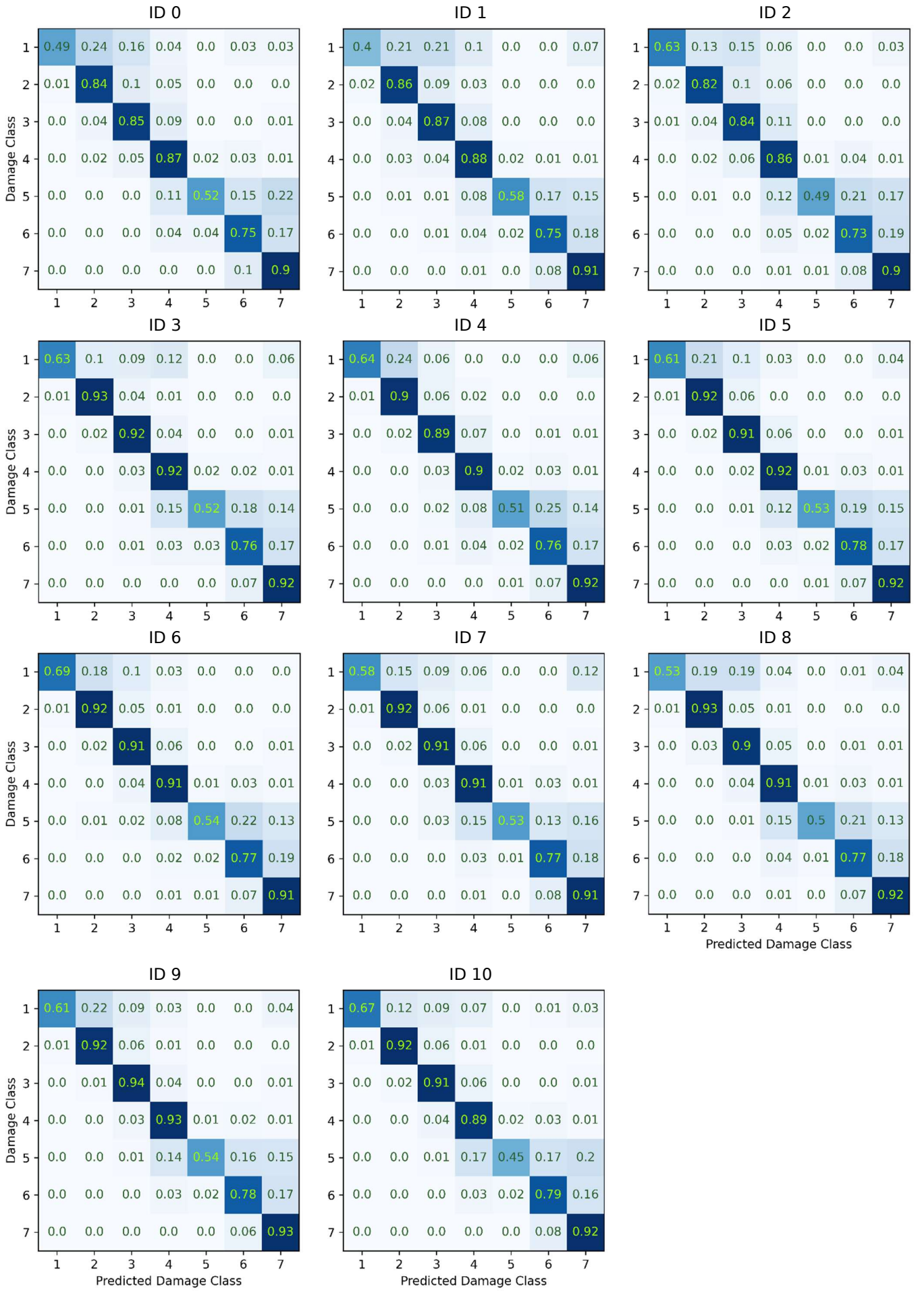
Figure S1. Normalized confusion matrices for the different models (ID as in Figure 1 of the paper). The numbers in the cells indicate the relative hit rate.
