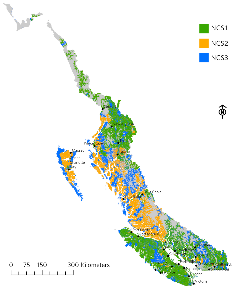
Supplemental Fig. 2 Natural Climate Solution (NCS) Action Category map for coastal temperate rainforests of British Columbia, Canada. NCS1 is available for action. NCS2 is not currently available for action. NCS3 is protected. Grey areas are non-forested.
