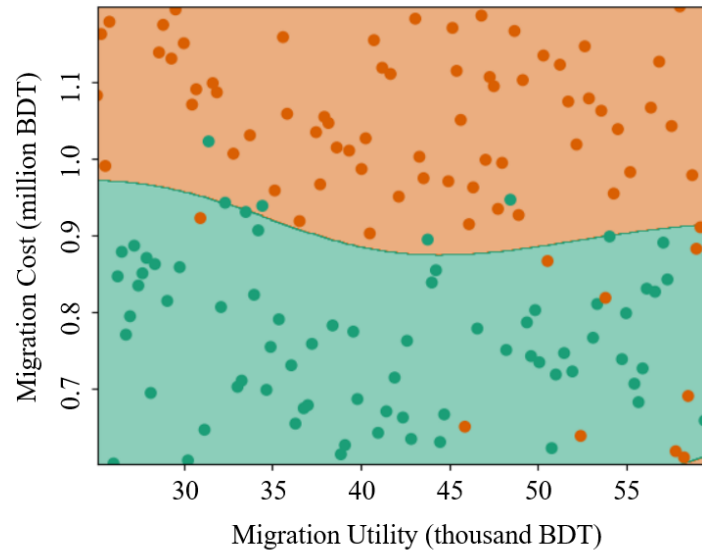
Figure S1: Parameter combinations of migration utility and migration threshold run for a Gini coefficient of 0.25 and SVM predicted successes of the parameter space for both patterns of interest. Points show parameter combinations sampled in the numerical experiments with green points indicating successful pattern replications and orange points indicating failed pattern replications. Colors show SVM predictions where green represents predicted success and orange represents failure.
