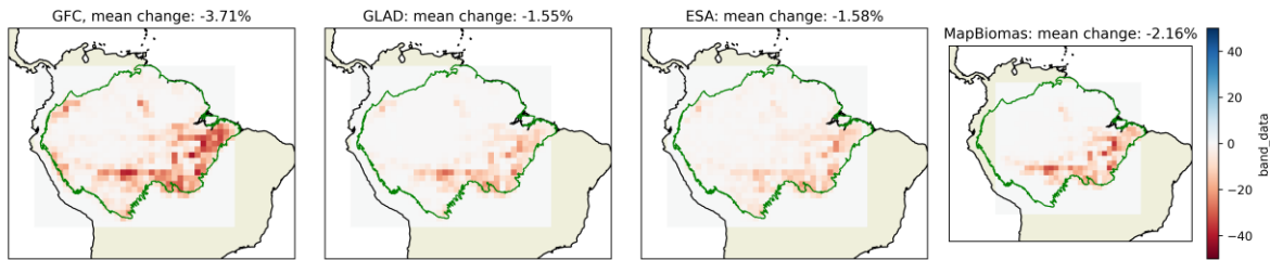
Figure S1. Change in Amazon biome forest cover between 2001 and 2020 in several land cover datasets; Global Forest Change (GFC), Global Land Analysis and Discovery (GLAD), European Space Agency (ESA) and Mapbiomas.
