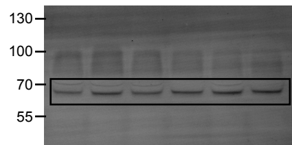
anti-pAKT
