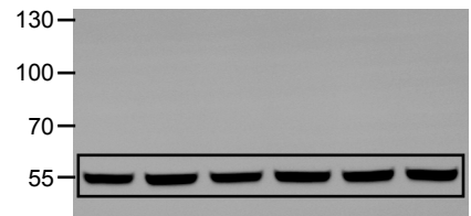
anti-Tubulin
