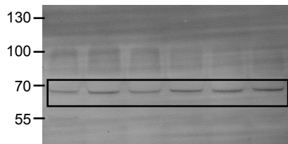
anti-AKT
