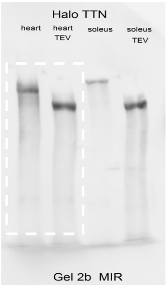
PVDF coomassie stain
