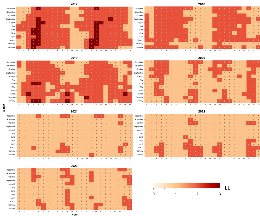
Supplementary figure 2. Heat maps of the average number of AIS data anomalies per hour per vessel for LL at 120 minutes intervals.
